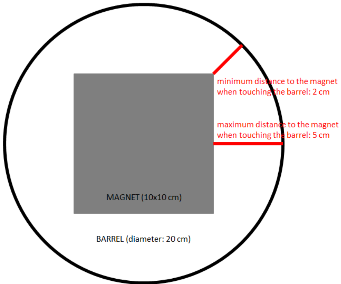
ESM Fig. 2 Sketch of the barrel containing the neodymium block (view from above). When touching the barrel, the distance to the magnet is 2-5 cm depending on the position.
