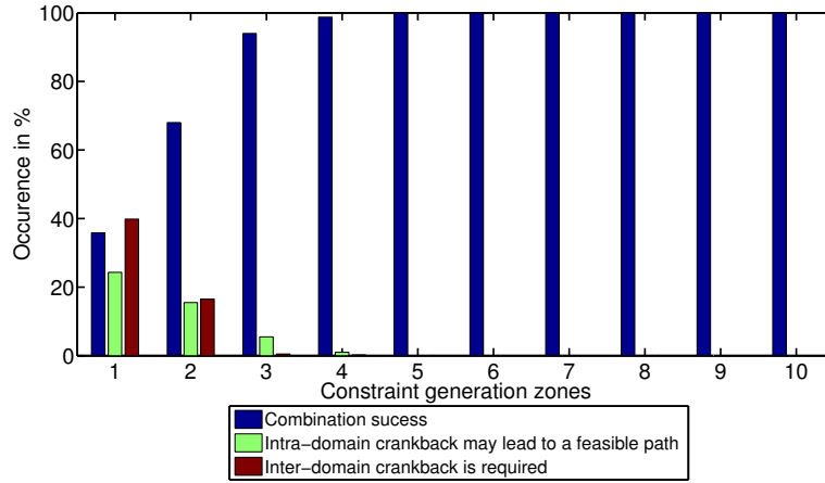
Fig. 6 Domain D_4 : Success rate of the combination procedure, percentage of requests requiring intra-domain crankback, and percentage of requests requiring the inter-domain crankback.
