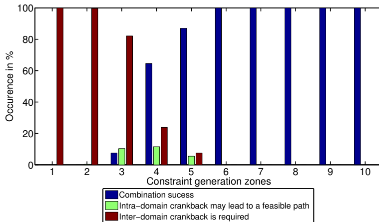
Fig. 7 Domain D_5 : Success rate of the combination procedure, percentage of requests requiring intra-domain crankback, and percentage of requests requiring the inter-domain crankback.
