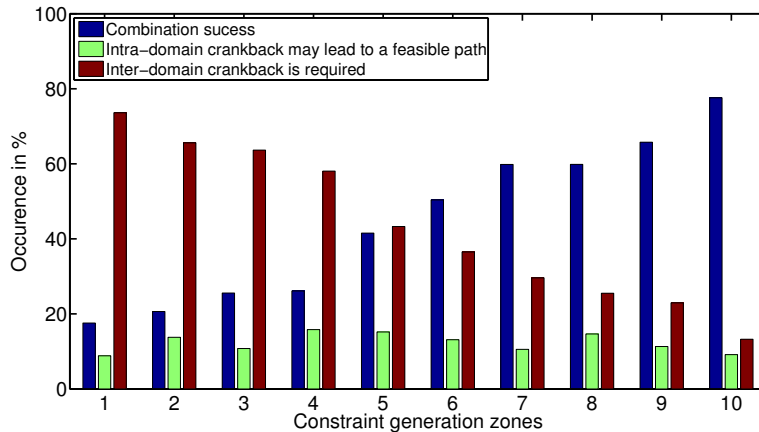
Fig. 8 Domain D_3 : Success rate of the combination procedure, and percentage of requests requiring intra-domain, and percentage of requests requiring the inter-domain cranking back.
