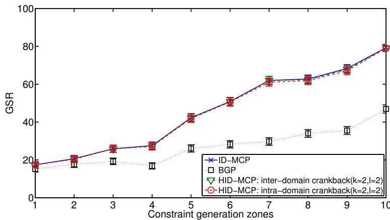
Fig. 11 Comparison of the global success rate of the algorithms in the SYM-CORE topology.
