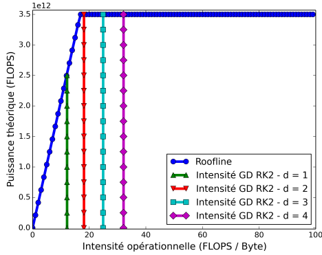
Figure 9: Roofline model and DG method. Abscissa: computational intensity I (FLOP/B). Ordinate: Algorithm perfs (TFLOP/s).
