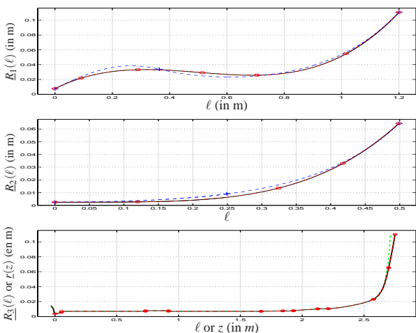
Figure 1: Test profiles \underline{R}_k (-). For \underline{R}_1 and \underline{R}_2 : examples of optimal approximation with N = 2 , N = 4 and N = 6 pieces of pipes (- - + and - - o). Original bore r_3(z) (- - -), \underline{R}_3(\ell) (-) and approximation with N = 11 pieces of pipes (- - o).
