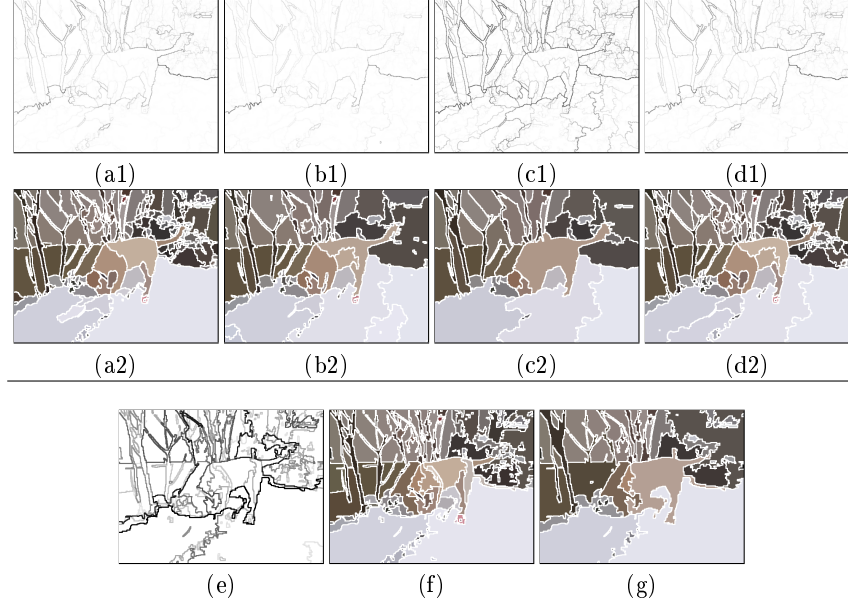
Fig. 3. Top, image segmentation of “Custard” using gaussian region model SW, where the first row is pdf(x) and second row the segmentation obtained at a given probability contrast: (a) using only color mean [12], (b) Bhattacharyya distance, (c) Hellinger metric distance, (d) Wasserstein metric distance. The number of realization is M = 50 and the number of random markers at each realization is N = 200 germs. Bottom, image segmentation of “Custard” using statistical region merging (SRM) [15]: (e) sum of contours obtained from SRM using nine values of Q (256, 128, 64, 32, 16, 8, 4, 2, 1), (f) segmentation for Q = 128 and (g) for Q = 32 .
