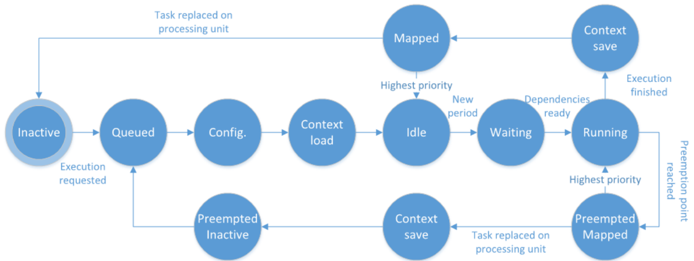
Fig. 5. Task finite-state machine
