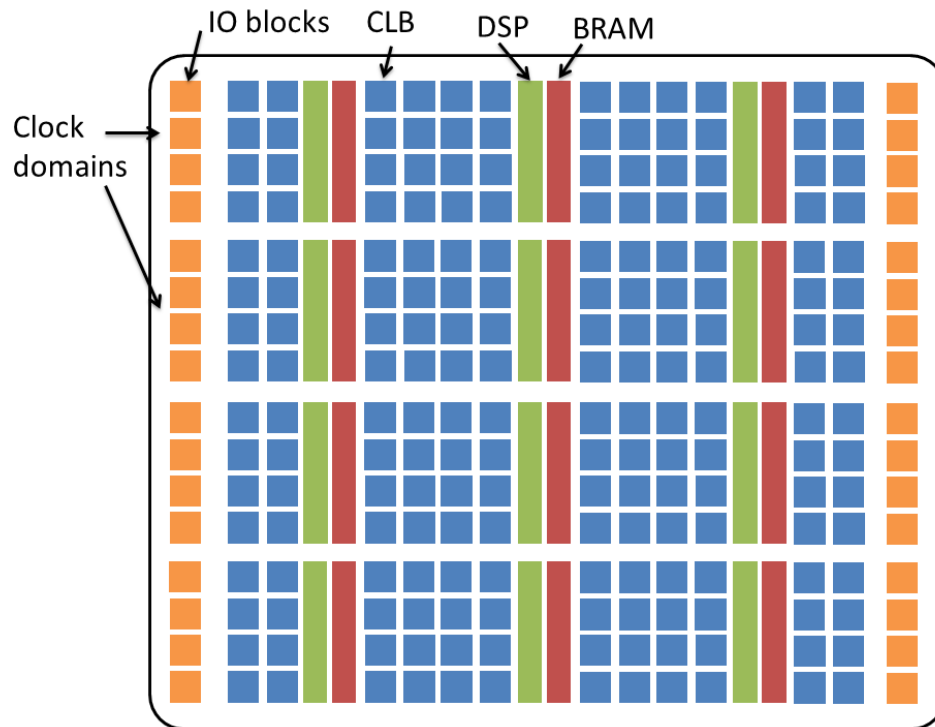
Fig. 1. Physical disposition of resources inside an FPGA
