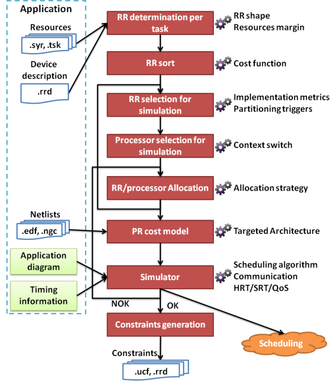
Figure 6: FoRTReSS flow
