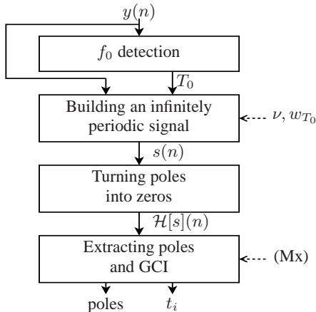
Figure 1: General scheme of the all-pole causal/anticausal decomposition algorithm
