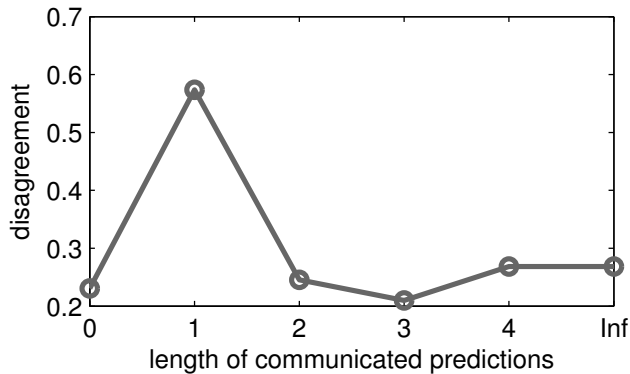
Figure 4: Influence of the maximal prediction length (“Inf” means it is not limited).
