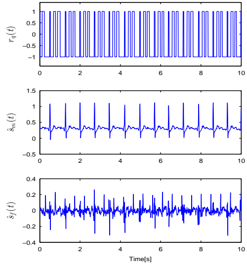
Fig. 3: Extraction of fetal ECG using a 1-bit reference with Gasussian process: r(t) is the thoracic reference, \hat{s}_m(t) is the maternal estimation, and \hat{s}_f(t) is the fetal estimation.
