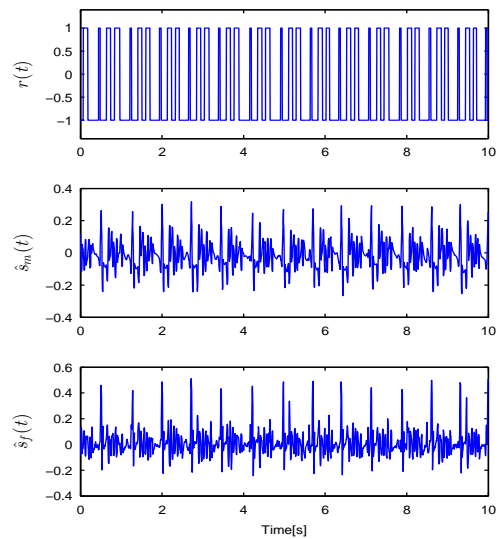
Fig. 5: Extraction of fetal ECG using a 1-bit reference with the adaptive filter: r(t) is the thoracic reference, \hat{s}_m(t) is the maternal estimation, and \hat{s}_f(t) is the fetal estimation.
