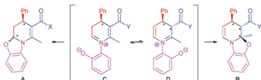
Scheme 2 Rationale for the control of the MCR's regioselectivity.
