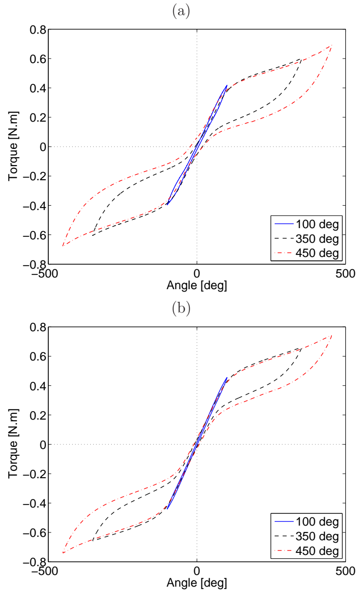
Figure 4: Quasi-static tests: Torque versus angle of torsion for specimen 1(a) and 2(b) at three different amplitudes (100, 350 and 450 degrees), at room temperature (24°C).
