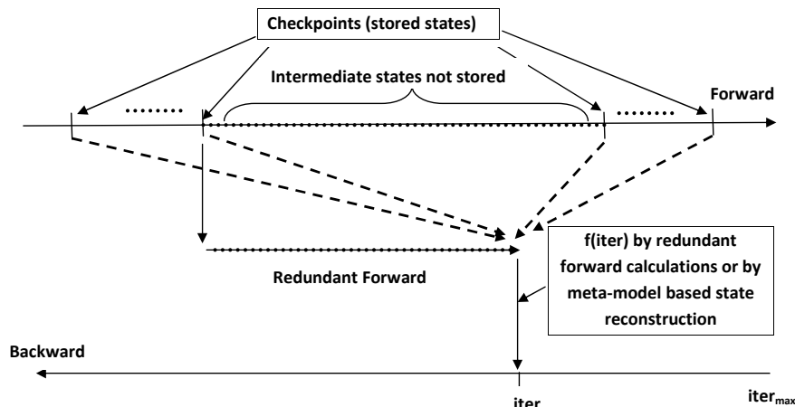
FIGURE 1. Sketch of our forward/redundant forward/backward combination, or when the redundant forward is replaced by a meta-model based reconstruction of non available intermediate states using checkpoint states.
