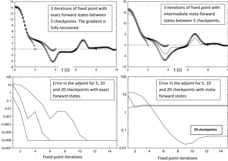
FIGURE 6. Parallel fixed point iterations of partial backward accumulation with meta-forward states described in 6.4. Upper left: with 5 checkpoints and exact forward states the gradient is fully recovered after 3 iterations of the fixed point algorithm. Upper right: the error in the gradient is due to the forward states between checkpoints based on a meta-model. Lower-left: error \varepsilon_b by (6.9) during fixed point iterations for 5, 10 and 20 checkpoints. Lower-right: same but with meta-forward states. One sees that a compromise can be found with 20 checkpoints between accuracy, absence of redundant calculations and checkpoints storage.
