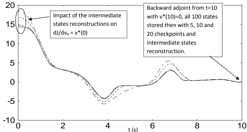
FIGURE 4. Model problem 7: full adjoint versus 5, 10 and 20 uniform checkpoints with the intermediate states reconstructed from these by a linear interpolation.
