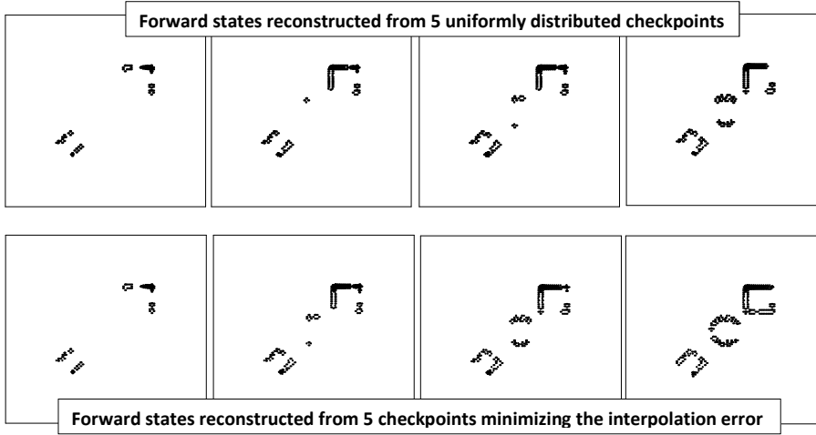
FIGURE 9. Contour identification from partial macroscopic field observation. Four snapshots of dJ/d\psi at iterations 5, 10, 15 and 20 of the parallel fixed point partial reverse accumulation to be compared to the full gradient presented in figure 8. The forward states are either reconstructed from 5 uniformly distributed checkpoints (upper) and when the checkpoints are distributed in order to reduce the interpolation error between \mathbf{f} and \pi_\delta \mathbf{f} .
