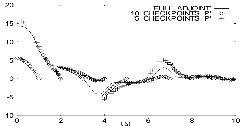
FIGURE 5. Same than figure 4 but with partial reverse accumulation and dynamic reallocation of the checkpoints. The same intermediate states reconstruction has been applied.
