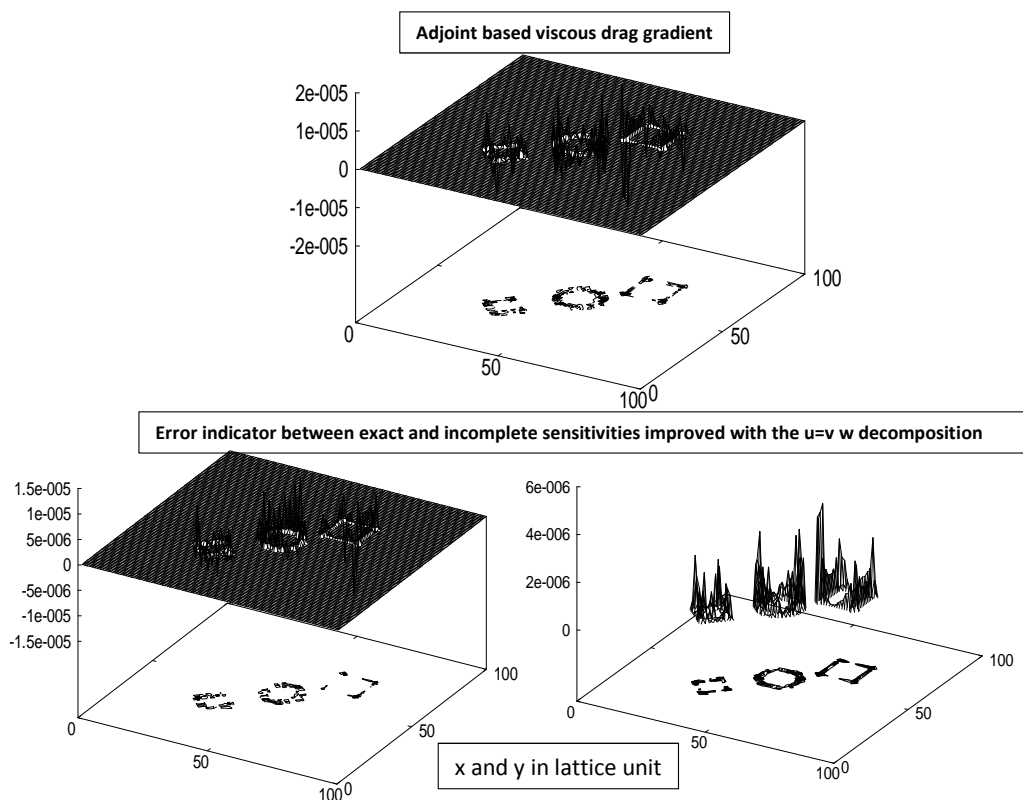
FIGURE 12. Top: viscous drag sensitivity \nabla_\psi C_d^v(t) with full adjoint. Lower-left: Local error between the full and incomplete evaluation of the gradient by indicator \eta from (9.3). Lower-right: same but taking advantage of decomposition (9.5).
