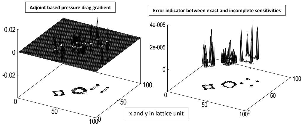
FIGURE 10. Left: pressure drag sensitivity \nabla_\psi C_d^p(t) with full adjoint. Right: Local error between the full and incomplete evaluation of the gradient by indicator \eta from (9.3).
