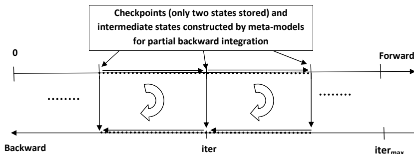
FIGURE 2. Partial forward/backward accumulation with only two checkpoint states stored and dynamically erased.
