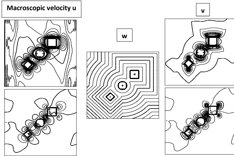
FIGURE 11. A snapshot of the macroscopic velocity u and its decomposition from (9.5).
