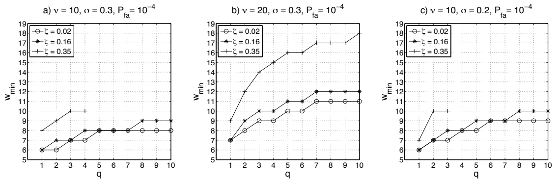
Figure 5: Theoretical conditions of detectability expressed in term of minimum length of detectable click train ( w_{min} ) as a function of the proportion of extra pulse q and for jitter width \zeta = 0.02, \zeta = 0.16 and \zeta = 0.35 . Parameters used to built the time-ICI map are: a) (\nu, \sigma, P_{fa})=(10, 0.3, 10^{-4}) ; b) (\nu, \sigma, P_{fa})=(20, 0.3, 10^{-4}) ; c) (\nu, \sigma, P_{fa})=(10, 0.2, 10^{-4}) .
