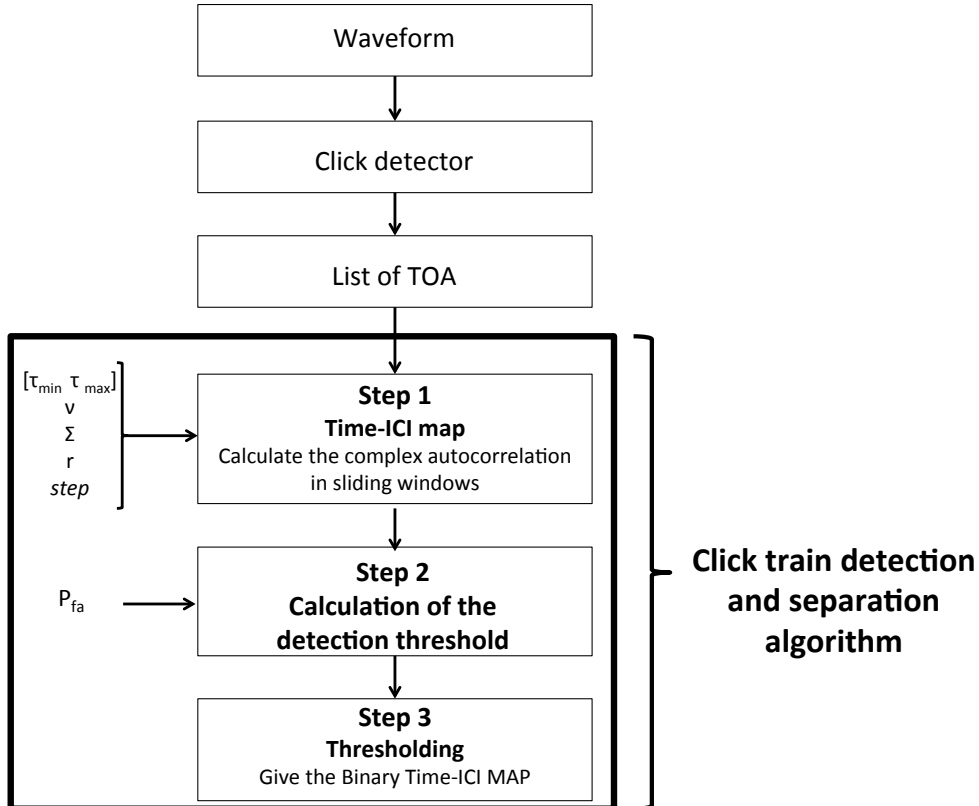
Figure 1: Signal processing steps of the proposed algorithm. The seven parameters needed to build the time-ICI map and perform the detection of the click trains are: [\tau_{min} \tau_{max}] : the expected minimum and maximum ICI values; r : the resolution of ICI bins; \nu : the number of periods with ICI equal to \tau contained in the window W(t, \tau) ; step the size of the sliding step of the time window along the pulse train; \sigma : the upper limit of the jitter in ICI bins b_k ; P_{fa} : the targeted probability of false alarm.
