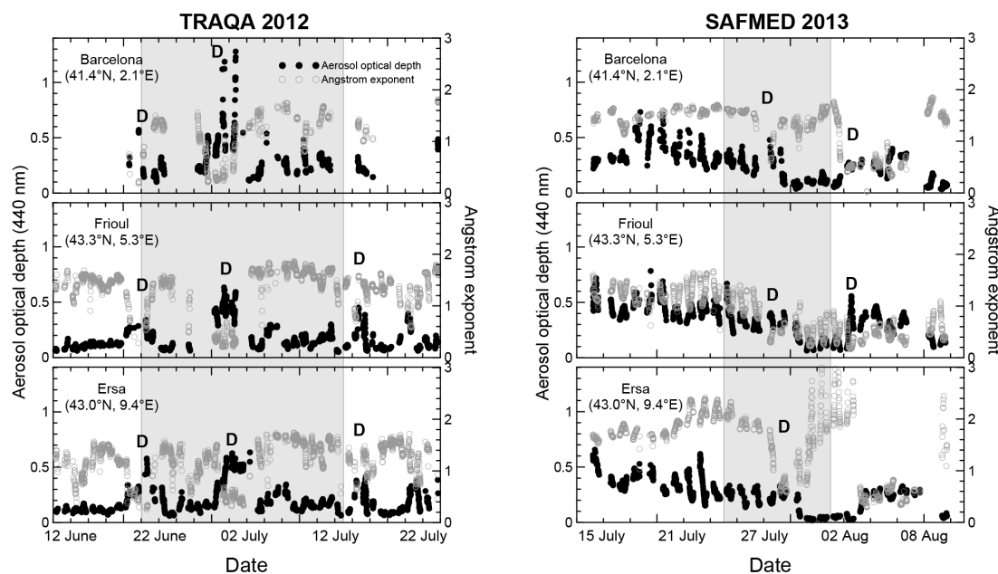
Figure 2. Aerosol optical depth at 440 nm ( \tau ) and Ångström exponent ( \alpha ) measured at the Barcelona, Frioul, and Ersá AERONET stations during the TRAQA 2012 (left panels) and the SAFMED 2013 (right panels) campaigns. The time period for the different plots is \pm 10 days around the beginning/end of the two campaigns (data for the Barcelona station are not available over the entire 2012 period). The label D indicates the days affected by Saharan dust.
