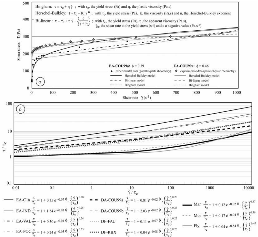
Figure 6. Fitting curve for the (a) COU99 material and (b) master curves of the landslides and in situ deposits.
