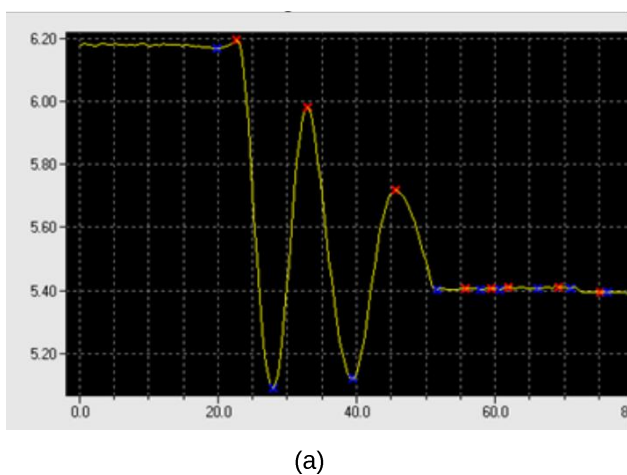
Figure 3 : (a) GaAs grating profile evolution for different etching times. (b) : Linear temporal evolution of the etch depth vs time
