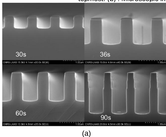
Figure 3 : (a) GaAs grating profile evolution for different etching times. (b) : Linear temporal evolution of the etch depth vs time
