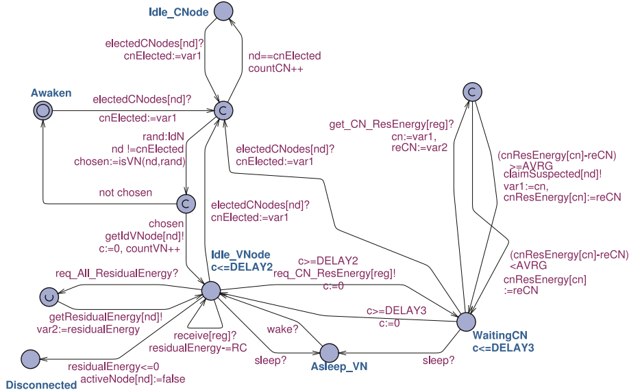
Figure 9: UPPAAL automaton of the vNode role
