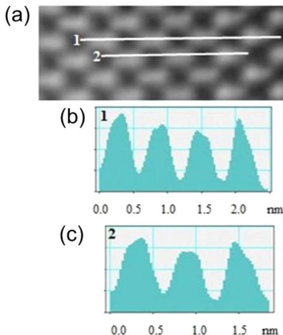
FIG. 4. (a) HAADF-STEM image of the CdSe on ZnTe interface (B). (b) Intensity profile along the line marked 1 in Figure 4(a), in the growth direction. (c) Intensity profile along the line marked 2 in Figure 4(a), in the growth direction.
