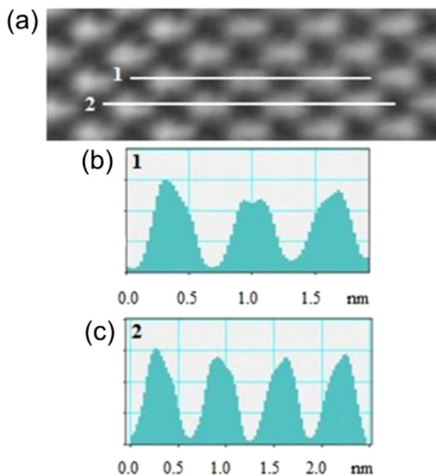
FIG. 2. (a) HAADF-STEM image of the ZnTe on CdSe interface (A) (b) Intensity profile along the line marked 1 in Figure 2(a), in the growth direction. (c) Intensity profile along the line marked 2 in Figure 2(a), in the growth direction.
