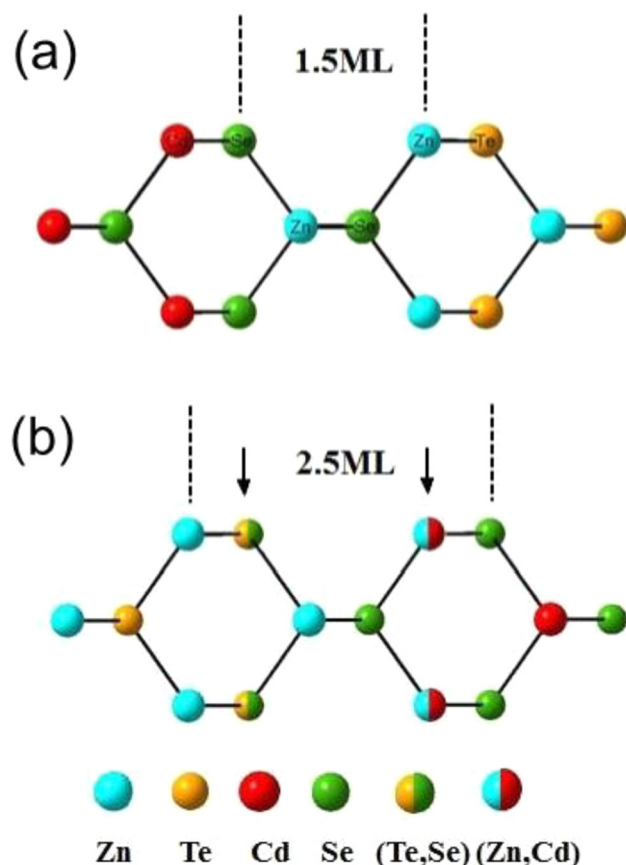
FIG. 3. Structural model projected along [110] for: (a) ZnTe on CdSe interface (A), (b) CdSe on ZnTe interface (B); the black arrows indicate the layers having cationic or anionic alloying.
