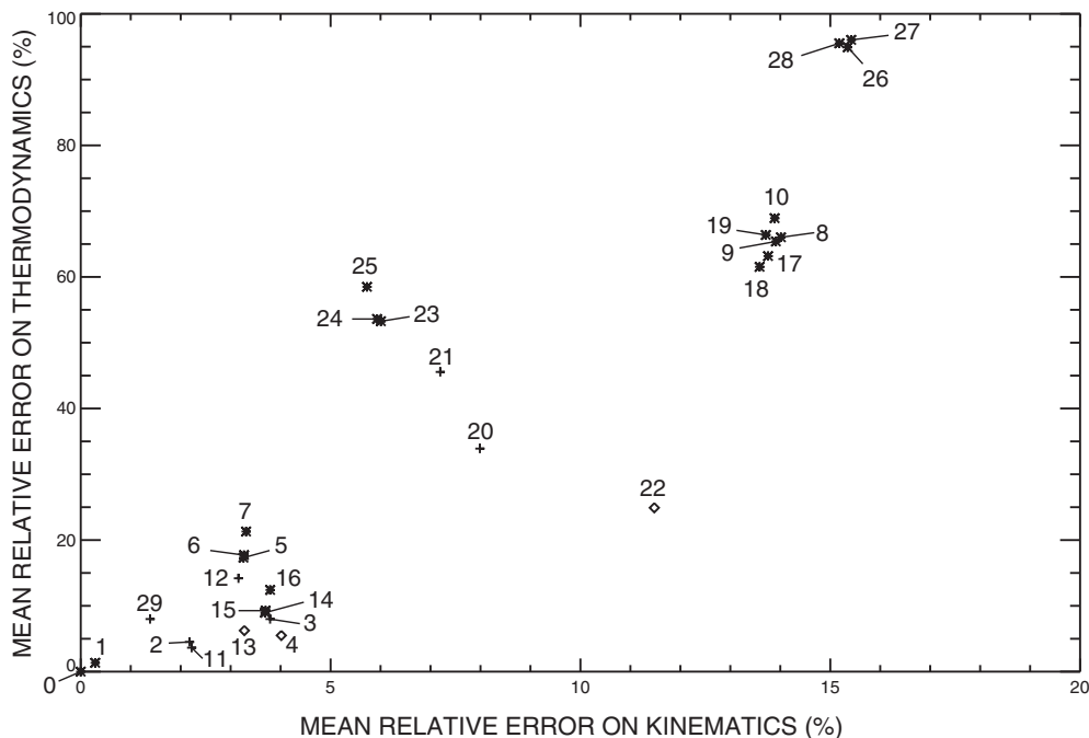
Fig. 7. Ranking of test experiments according to the mean relative errors made on kinematics (transfer intensities, mean positions at 27.8°S and 35°W and associated standard deviations) and on thermodynamics (inflowing and outflowing temperature and salinity fluxes for each transfer). The numbers and features of all test experiments are listed in Table 1. For easier readability, test experiments using W=0 , an isopycnal flow or the connection of salinity minima as a condition on the vertical velocity are shown with plus, star and diamond symbols, respectively.
