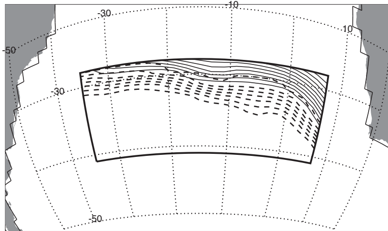
Fig. 6. Lagrangian horizontal streamfunction for the reference experiment using full information from the model velocity field. Solid contours: the volume transfer from 7°E to 27.8°S. Dashed contours: volume transfer from 7°E to 35°W. The contour interval is 0.5 Sv.
