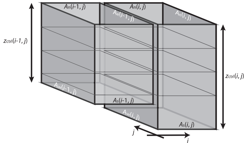
Fig. 2. Example of adjacent water columns over which the volume budget optimization is to be done.
