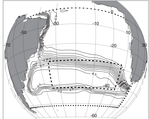
Fig. 5. Lagrangian horizontal streamfunction for the basin-wide experiment. The contour interval is 0.5 Sv. The domain over which the test experiments will be performed is framed with a dashed line.
