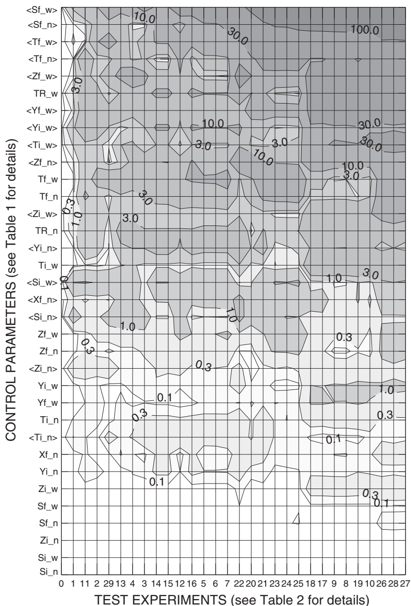
Fig. 8. Relative errors for each test experiment and each control parameter. The filled contours show the error intervals [0–0.1%], [0.1–0.3%], [0.3–1%], [1–3%], [3–10%], [10–30%], [30–100%], and [100–300%] with progressively darker shading. The code for the control parameters is the following: TR, X, Y, Z, T, and S refer to the intensity, longitude, latitude, depth, temperature, and salinity, respectively, for the transfers made either to the northern section at 27.8°S (suffix “_n”) or the western section at 35°W (suffix “_w”). For each transfer, each parameter (except TR) is tested both on the initial section at 7°E (“i”) and on the final section (“f”). The experiments and parameters have been sorted to make the plot more legible (see text for details).
