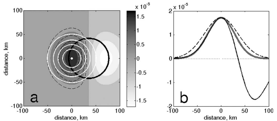
Figure 2. (a) The exact expression for the vertical velocity w \sim \frac{\partial H_m}{\partial r_m} \cos \theta_m ( V_m = 1 \text{ cm s}^{-1} , color, black dash contours) and its approximation with the radial symmetric form \sqrt{\frac{2}{e}} \frac{\Delta H}{R_m} e^{-\frac{\pi r^2}{2 R_m^2}} (white empty circles), thick black dash circle marks the isoline of the maximum meddy azimuthal velocity at the distance R_m/\sqrt{2} from the meddy center ( R_m = 30 km). (b) Same as Figure 2a but for the profiles \frac{\partial H_m}{\partial r_m} \cos \theta_m , passing through the center of the surface signal in the zonal (solid black line) and meridional (dashed line) directions. The radially symmetric profile of \sqrt{\frac{2}{e}} \frac{\Delta H}{R_m} e^{-\frac{\pi r^2}{2 R_m^2}} (grey solid line).
