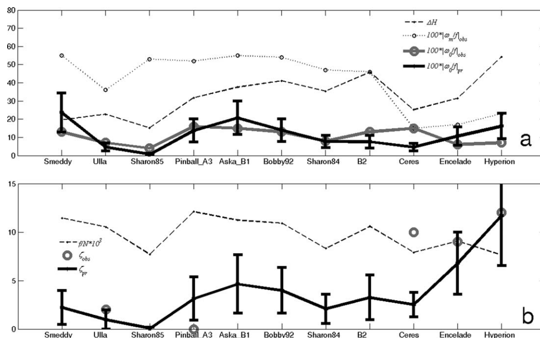
Figure 5. (a) Observed (solid grey line with circles) and predicted (solid black line with errorbars) are peak relative vorticities of meddy surface signals |\omega_0(0)| (s -1 ). Observed peak relative vorticity of meddies |\omega_m(0)| (s -1 ) is shown with dotted thin line with small circles, computed \Delta H —with dashed black line. (b) Observed (circles) and predicted (solid black line with errorbars) peak SLA over meddies and the climatic f/N ratio multiplied by 10^3 presented with dash thin line. The observed sea-level anomalies (SLA) are derived from AVISO altimetry data and are not available for the meddy observations before 1993.
