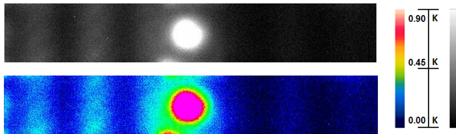
Fig. 9. Thermal image (heating) of the sample damaged at 250 MPa (black & white and colours).
