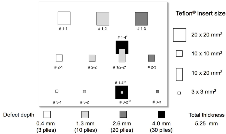
Fig. 1. Tested C/epoxy coupon: distribution of the artificial defects (manufacturing data, confirmed by ultrasonics scans).
