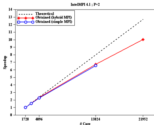
Figure 1: Taylor-Green Vortex DNS - Scalability for P = 2
