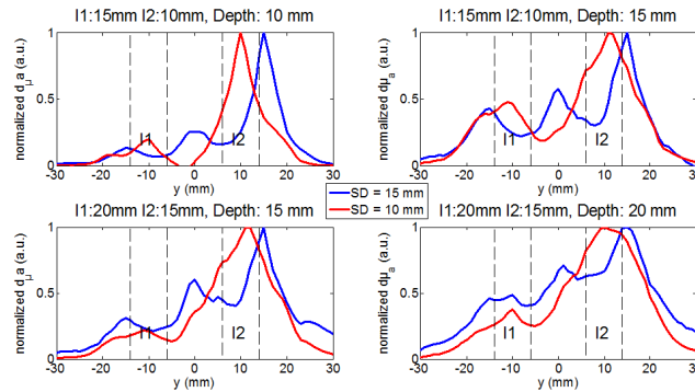
Fig. 7. d\mu_a profiles (normalized by maximum) along y axis at x = 0 and at the real depths of I1 and I2, extracted from Fig. 6. The dotted lines delimit the width of I1 and I2 along the y axis.
