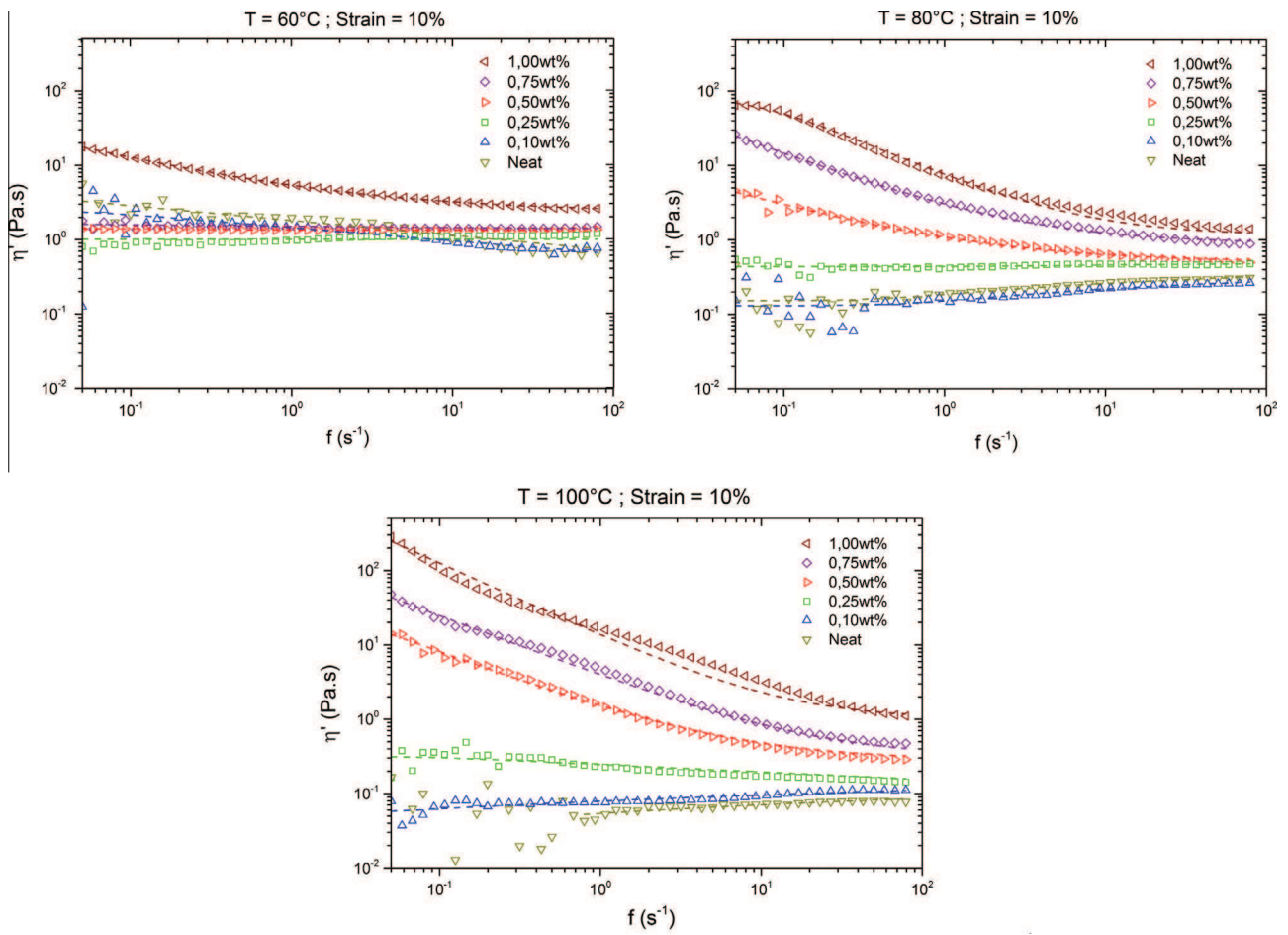
Fig. 3. Logarithmic frequency sweeps for neat and CNT doped epoxy (100 °C).
