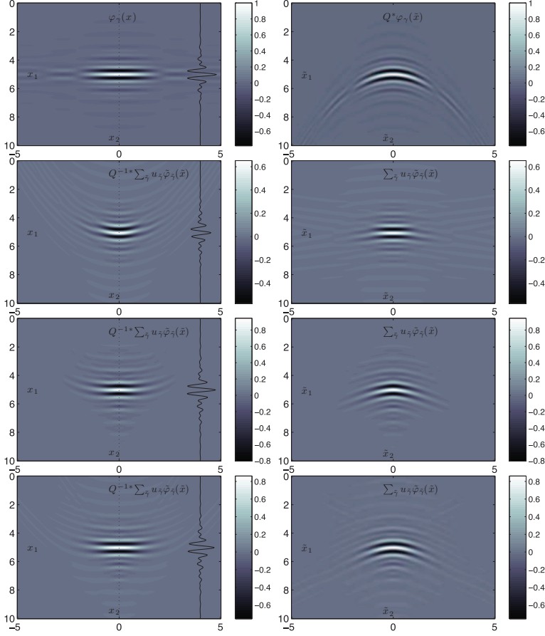
FIG. 3. Illustration of diffeomorphism Q , Q^{-1} and redecomposition for a wave packet \varphi_\gamma(x) at frequency scale k = 2 . Top row: \varphi_\gamma(x) (left) and pull back Q^*\varphi_\gamma(\tilde{x}) (right). Rows 2 to 4: Redecompositions \sum_{\tilde{\nu},k} u_\gamma \tilde{\varphi}_\gamma(\tilde{x}) of Q^*\varphi_\gamma(\tilde{x}) using 3, 7, and 9 boxes B_{\tilde{\nu},k} , respectively (right column), and the corresponding image Q^{*-1}(\sum_{\tilde{\nu},k} u_\gamma \tilde{\varphi}_\gamma)(x) under the action of Q^{-1} (left column). An insufficient number of boxes alters the amplitudes and the minimum phase property of wave packets. Increasing the number of boxes yields satisfactory results in an open neighborhood of (x_0, \xi_0) .
