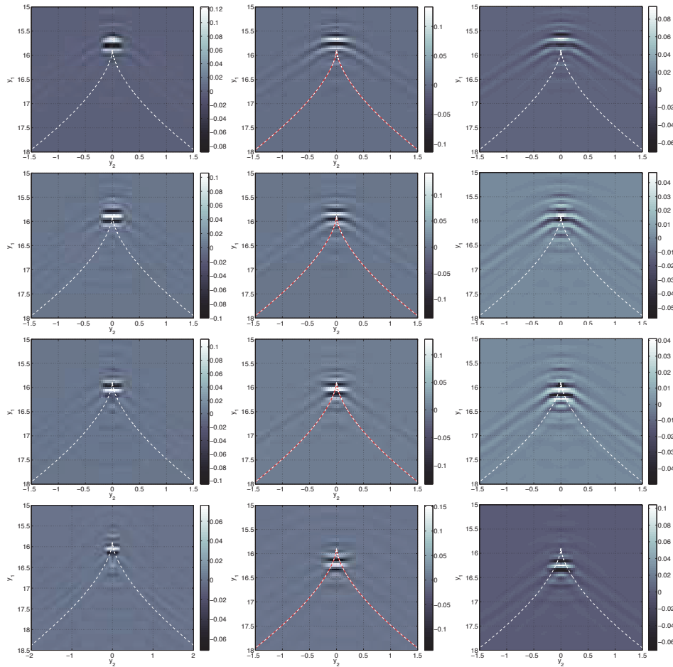
FIG. 9. Left column: Joint contribution of the operators F_i and F_{ij} acting on a wave packet \varphi_\gamma(x) at frequency scale k = 3 (compare with Figure 8(bottom left) for a wave packet at frequency scale k = 2 ). Center column: Time domain finite difference reference. Right column: The equivalent to the left column when using a separated representation with J_{\nu,k} = 11 terms. (Note that for computational reasons, only one box B_{\nu,k} has been used in the numerical evaluation of F_i and F_{ij} with J_{\nu,k} = 11 terms.)
