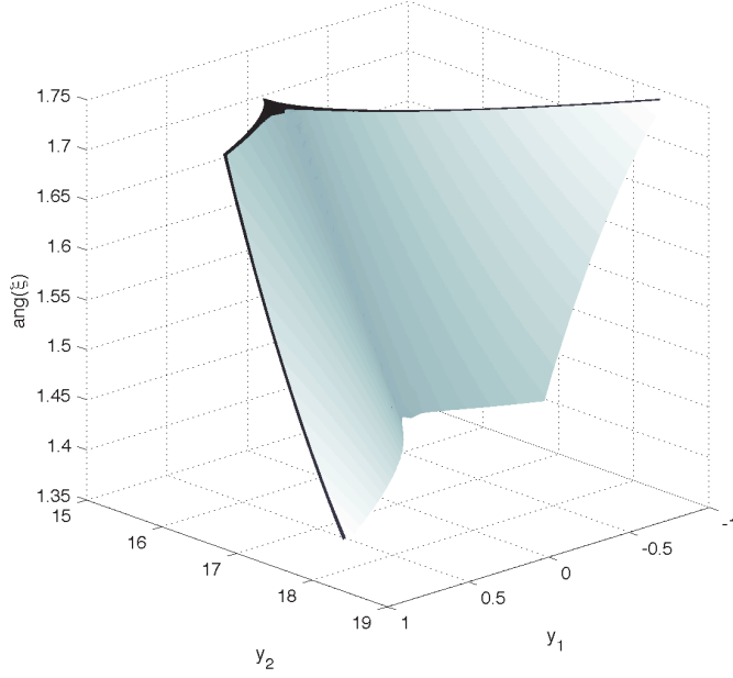
FIG. 2. Caustic surfaces \Xi(y, \xi) (dark gray) and \tilde{\Xi}(y, \xi) (light gray) of \Lambda and \tilde{\Lambda} corresponding to propagation through a low velocity lens (cf. section 5): The singular regions of \Lambda and \tilde{\Lambda} do not intersect.
