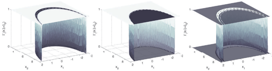
FIG. 5. Illustration of joint partition of unity for the partition functions and sets in Figure 4 for \xi_0 = 1.67 fixed: Slice of \bar{\Gamma}_i(x, \xi = \xi_0) (left), the admissible set U_{ij} and the associated partition function \bar{\Gamma}_{ij}(x(\tilde{x}, \tilde{\xi}), \xi(\tilde{x}, \tilde{\xi}) = \xi_0) (center), and the partition function \bar{\Gamma}_{ij}(x(\tilde{x}, \tilde{\xi}), \xi(\tilde{x}, \tilde{\xi}) = 1.67) for O_{ij} realizing the partition of unity with \bar{\Gamma}_i(x, \xi = \xi_0) .
