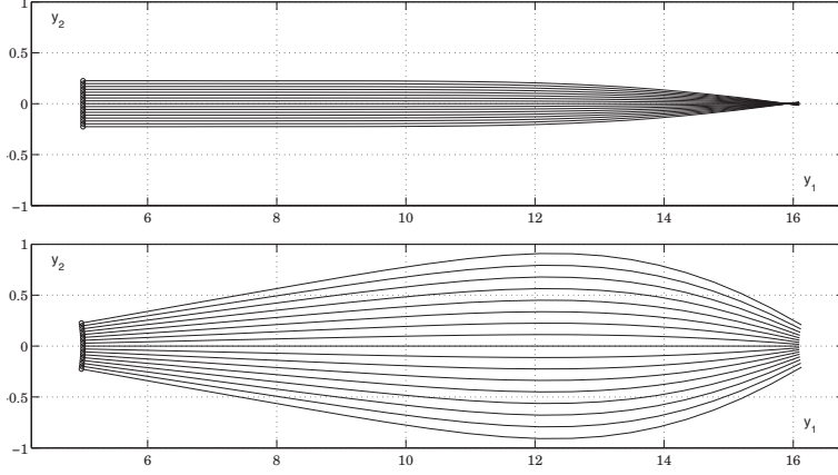
FIG. 1. Illustration of canonical relations \chi (top) and \tilde{\chi} (bottom) of operators F and \tilde{F} associated with a half-wave equation: (bi-)characteristics (“rays”) in y for initial conditions (x_2 = x_{2,0}, \xi = \xi_0) and (\tilde{x}_2 = \tilde{x}_{2,0}, \tilde{\xi} = \tilde{\xi}_0) , respectively, for evolution through a low velocity lens (see section 5). The black circles on the left indicate the conjugate points corresponding to the initial conditions.
