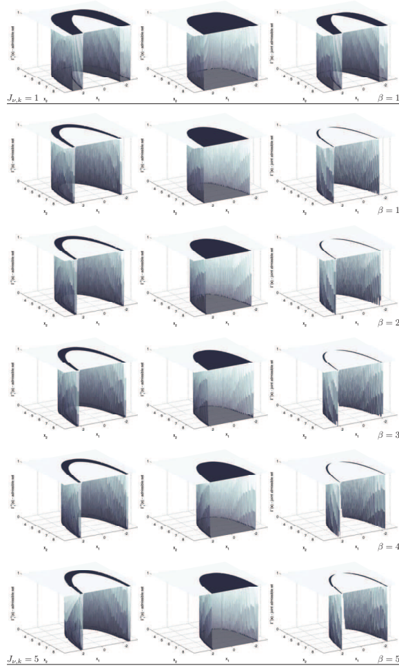
FIG. 7. Illustration of admissible sets and expansion functions \check{\Gamma}_1^\beta(y(x)) in (3.11) with J_{\nu,k} = 1 (top row) and J_{\nu,k} = 5 (lower rows) for the partition functions in Figure 4. Left column: The partition functions \bar{\Gamma}_i(y(x), \xi) , i = 1, 3 . Center column: The partition functions \bar{\Gamma}_i(y(\tilde{x}, \tilde{\xi}), \xi(\tilde{x}, \tilde{\xi})) , i = 2, j = 1 . Right column: The joint admissible sets induced by the partition of unity for the expansion functions plotted in the left and center columns.
