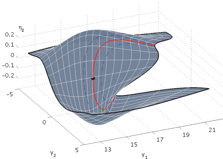
FIG. 6. Projection \bar{\Lambda}(y, \eta_2) of a slice \xi = \xi_0 of the canonical relation \Lambda associated with a half-wave equation in the vicinity of a caustic (red solid line; the blue dashed lines indicate the neighborhood of the singularity) caused by a low velocity lens. The white solid lines are connected to a regular grid in x by bicharacteristics. The black dot indicates the center of an open neighborhood of conjugate points (x_0, \xi_0) \mapsto (y_0, \eta_0) for which the projection onto standard microlocal focal coordinates (y, \xi) is not diffeomorphic.
