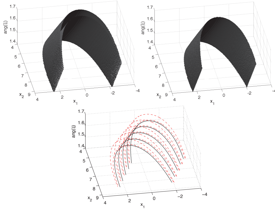
FIG. 4. Top left: Iso-amplitude surface of the partition functions \bar{\Gamma}_i(x, \xi) , i = 1, 3 , associated with Q_i = \mathbb{I} : the joint admissible set O_1 \cup O_3 comprises the exterior of the two sheets. Top right: Iso-amplitude surface of \bar{\Gamma}_{ij}(x(\tilde{x}, \tilde{\xi}), \xi(\tilde{x}, \tilde{\xi})) for \xi_0 = \pi/2 , x_{2,0} = 0 , and \alpha = 1 ( i = 2, j = 1 ): the admissible set O_{ij} contains the region on the back of the sheet. Bottom: Boundaries \partial O_i , i = 1, 3 (dashed curves), and \partial O_{ij} , i = 2, j = 1 (solid curves), of the admissible domains: clearly, the joint admissible set O_1 \cup O_3 \cup O_{21} covers \Lambda .
