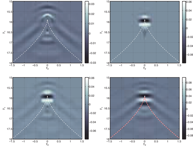
FIG. 8. Illustration of operator action on a wave packet \varphi_\gamma(x) at frequency scale k = 2 : Contribution of operators F_i ( i = 1, 3 ) associated with Q_i = \mathbb{I} (top left), contribution of operator F_{ij} ( i = 2, j = 1 ) with diffeomorphism parameters ( \xi_0 = \pi/2, x_{2,0} = 0, \alpha = 1 ), resolving the singularity in the tip of the caustic (top right), and joint action of F_i and F_{ij} (bottom left). Time domain finite difference reference (bottom right). In the operator computation, we consider 9 boxes B_{\bar{\nu},k} and a separated representation with J_{\nu,k} = 1 term.
