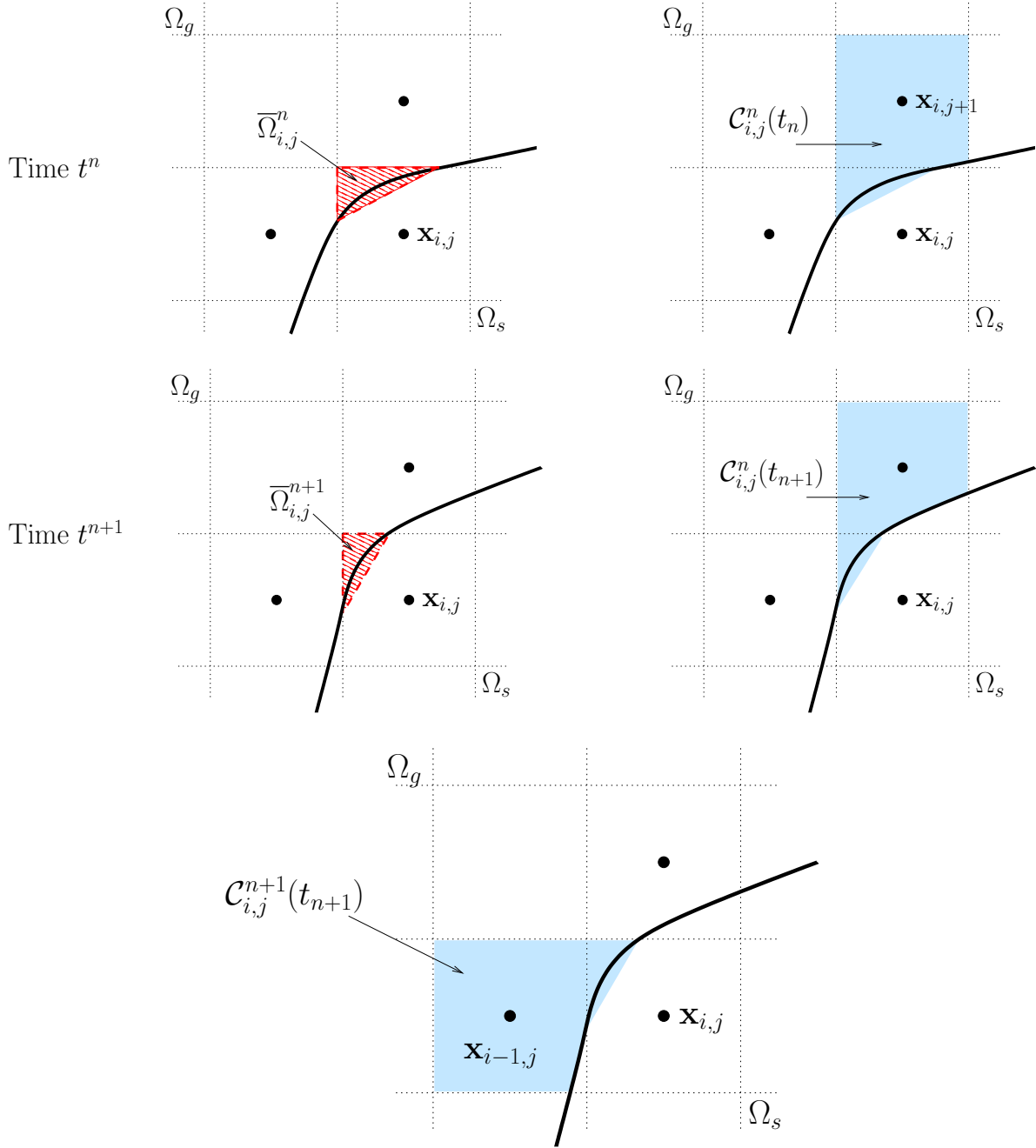
Figure 3: Top-Left: the virtual cell \bar{\Omega}_{i,j}^n (hatched) has to merge with \bar{\Omega}_{i,j+1}^n because |L_{i,j+1}^n| > |L_{i-\frac{1}{2},j}^n| . Top-Right: this results in the control volume \mathcal{C}_{i,j}^n(t^n) , in blue. Middle-Left: at time t^{n+1} , the solid boundary has slightly turned counter clock-wise and the virtual cell \bar{\Omega}_{i,j}^{n+1} is smaller. Middle-Right: the control volume at this time now is \mathcal{C}_{i,j}^n(t_{n+1}) , in blue. Bottom: since the larger edge of the virtual cell \bar{\Omega}_{i,j}^{n+1} now is |L_{i-\frac{1}{2},j}^{n+1}| , it has to merge with \bar{\Omega}_{i-1,j}^{n+1} , and this results in the new control volume \mathcal{C}_{i,j}^{n+1}(t_{n+1}) , which is different from \mathcal{C}_{i,j}^n(t_{n+1}) .
