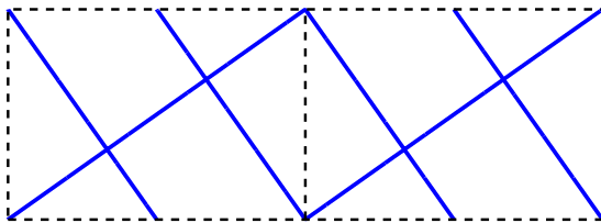
(a) A nodal 6-partition of \mathbb{T}(2, 1/\sqrt{2}) (associated with \cos(3\pi x) - \cos(\pi x) \cos(2\sqrt{2}\pi y) + \sin(\pi x) \sin(2\sqrt{2}\pi y) ).
