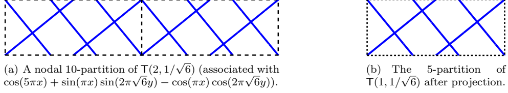
Figure 3: Construction of a 5-partition of T(1, 1/\sqrt{6}) .
