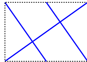
(b) The 3-partition of \mathbb{T}(1, 1/\sqrt{2}) after projection.
