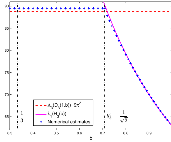
Figure 6: Upper bounds of \mathfrak{L}_3(\mathcal{T}(1, b)) for b \in \{j/100; j = 30, \dots, 100\} .
