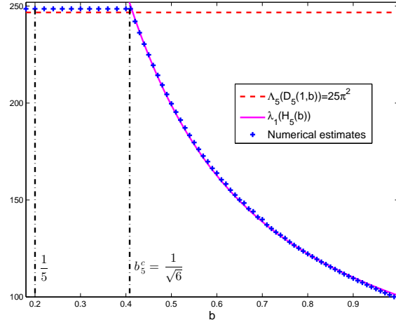
Figure 10: Upper bounds of \mathfrak{L}_5(\mathsf{T}(1, b)) for b \in \{j/100; j = 18, \dots, 100\} .
