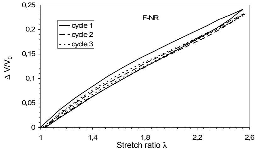
Fig. 6. The first mechanical cycle in F-NR: volume variation decreases with the cavity size, and melting of crystallites starts. The fact that for a given stretch ratio the volume is superior during loading than during unloading is mainly explained by the difference in the kinetics of crystallization and melting. During unloading, from \lambda = \lambda_{melting} , the melting of crystallites is complete, and volume decrease is only due to cavities closing. This explains why the curve slope increases.
