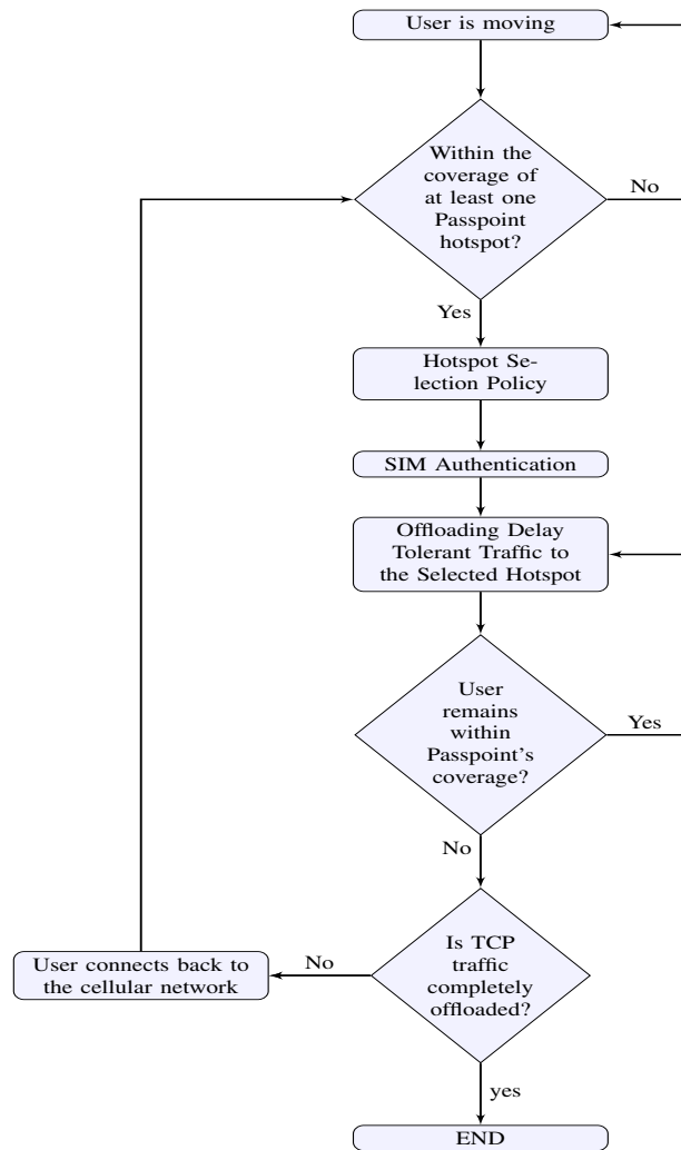
Figure 5: Offloading algorithm.
