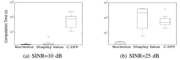
Fig. 4. Computation time comparison for the two datasets.
