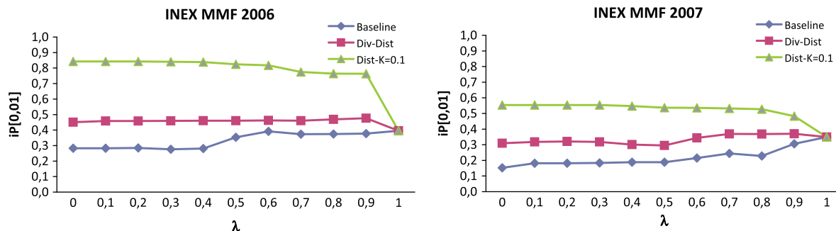
Fig. 12. Impact of the factor Dist(em_i, Anc) according to the iP[0.01] metric.
