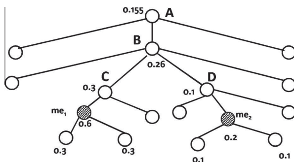
Fig. 3. Using the factor Dist(me_i, mf) to compute ancestors scores.
