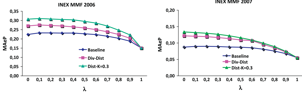
Fig. 8. Comparison between combination with and without the factor Dist(im_i, Anc/Desc) .
