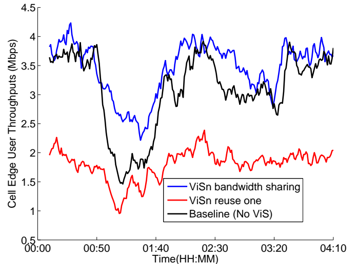
Fig. 7. Cell edge user throughputs evolution over time
