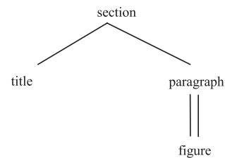
Fig. 4 – A twig query.
