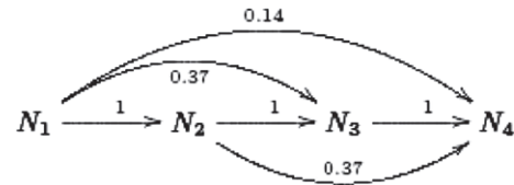
Fig. 10 – Original and final paths. Original paths are weighted with 1.
