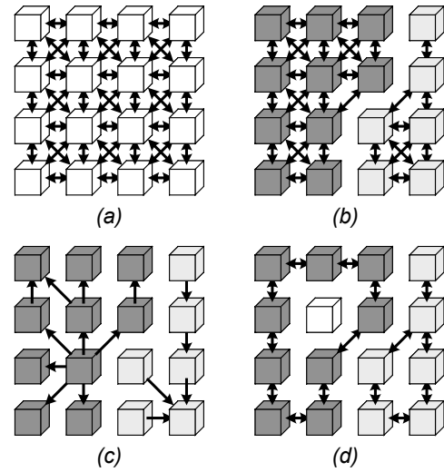
Fig. 7 Different mgraphs configurations: (a) Full graph (b) Region graph (c) Oriented trees (d) Edges graph
