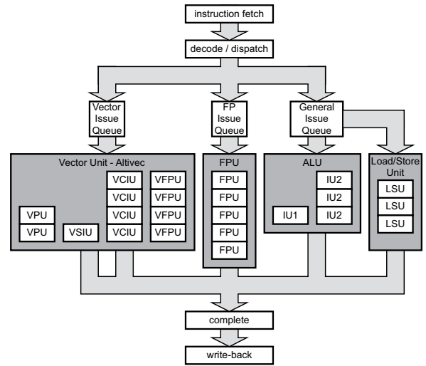
Fig. 2 PowerPC G4 pipeline
