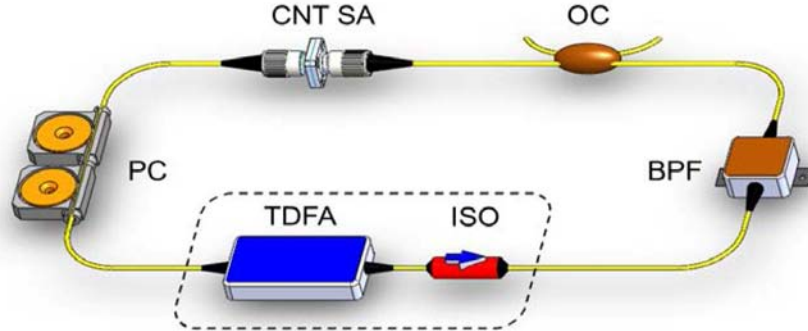
Fig. 1. Schematic of the mode-locked oscillator. T DFA: thulium-doped fiber amplifier, ISO: isolator, BPF: bandpass filter, OC: fiber output coupler, CNT SA: carbon nanotube saturable absorber, PC: polarization controller.
