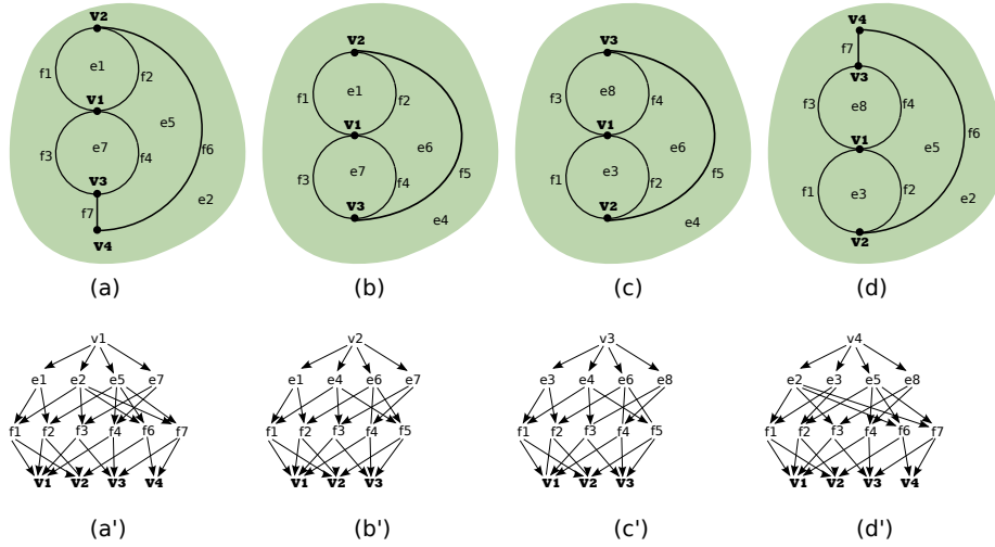
Figure 9: A regular CW -complex C , which dual is represented in Fig. 8. C is made of four volumes v_1..v_4 , eight faces e_1..e_8 , seven edges f_1..f_7 and four vertices V_1..V_4 . On (a) – (d), the boundaries of volumes v_1, v_2, v_3, v_4 ; on (a') – (d'), the corresponding incidence graphs.
