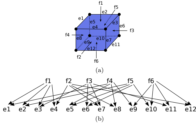
Figure 2: (a) A cube v . (b) The suborder \alpha(v) restricted to 1- and 2-dimensional cells is connected.
