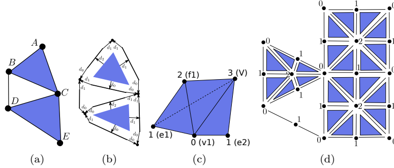
Figure 5: (a) A representation of an abstract simplicial complex which contains 3 main cells (2 triangles and an edge). (b) A corresponding semi-simplicial set. (c) The order complex corresponding to the order depicted on Fig. 1(e). It contains two main simplices corresponding to (v1, e1, f1, v) and (v1, e2, v) . (d) The order complex corresponding to the chains of surfaces depicted on Fig. 1(b) and to the cmap depicted on Fig. 4(h).
