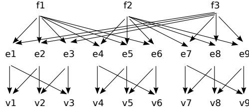
Figure 3: This incidence graph encodes a combinatorial cell complex as defined by Basak [4], but the boundary of each 2-cell is not connected. Hence it is no chain of surfaces.
