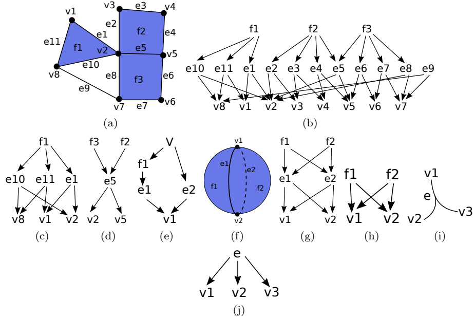
Figure 1: (a) A subdivision of a part of the plane; the main cells are faces f_1 , f_2 and f_3 , and edge e_9 . (b) The corresponding DAG. (c) The suborder corresponding to \alpha(f_1) . (d) The suborder corresponding to \theta(e_5) . (e) A non closed order, since the ranks of e_2 and v are equal to 1 and 3, and no 2-dimensional cell is incident to both e_2 and v . (f) A subdivision of a sphere. (g) The corresponding 2-surface. (h) |\theta^\square(e_1)| = |\theta^\square(e_2)| is a 1-surface. (i) edge e is incident to vertices v_1 , v_2 and v_3 . (j) The corresponding order.
