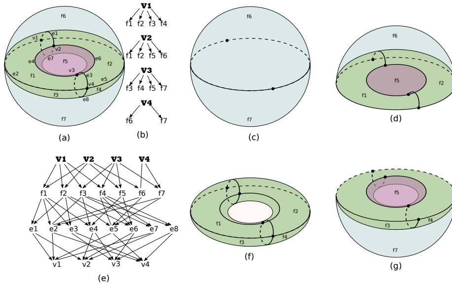
Figure 8: (a) A representation of a subdivision C^d made of four volumes. (b) The faces incident to each volume. The boundary of volume V1 (resp. V2 , V3 , V4 ) is represented in (f) (resp. (d), (g), (c)). The incidence graph of C^d is represented in (e).
