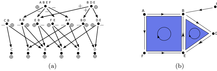
Figure 6: (a) Orientation of the cells of a 2-dimensional chain of surfaces. (b) Corresponding orientation of the cells of the associated subdivision.
