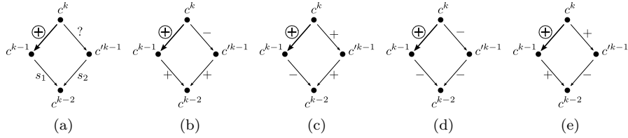
Figure 7: Inductive orientation process according to the switch-property .
