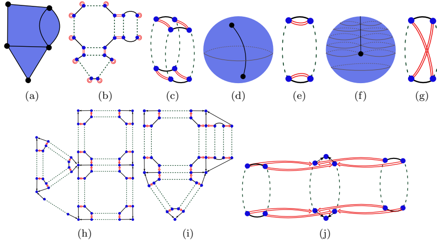
Figure 4: (a) A subdivision of a part of the plane. (b) The corresponding 2-gmap. Darts are represented by points, \alpha_0 by dashed lines, \alpha_1 by full lines, \alpha_2 by double lines. (c) The 2-gmap corresponding to the subdivision depicted on Fig. 1(f). (d) A subdivision of a sphere. (e) The corresponding 2-gmap. (f) A subdivision of the projective plane. (g) The corresponding 2-gmap. (h) The chain of maps corresponding to the subdivision depicted on Fig. 1(a). \sigma^1 is represented by arrows, \sigma^2 by double arrows. (i) The chain of maps corresponding to the 2-gmap depicted on Fig. 4(b). (j) The chain of maps corresponding to the 2-gmap depicted on Fig. 4(c).
