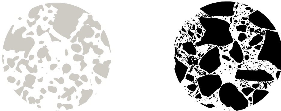
(a) Excursion set extracted from FIG. (16). (b) Segmented X-ray microtomography from Qier (2014).
