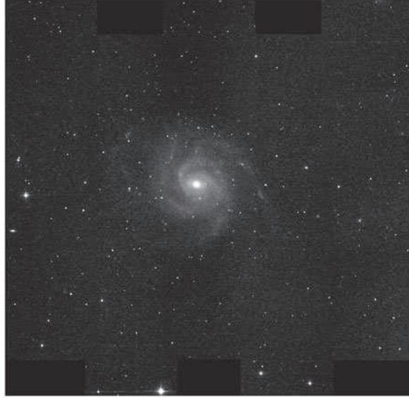
Fig. 11 The background-matched version of the mosaic
