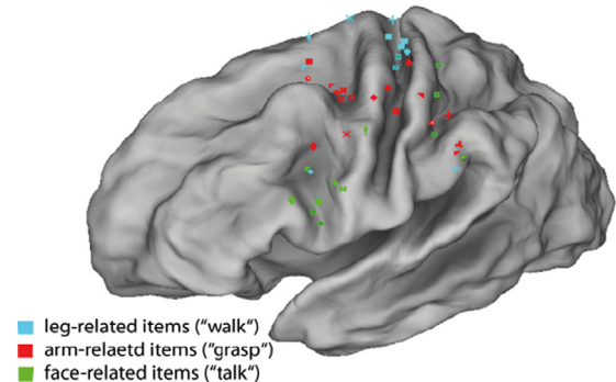
Fig. 7. Manifestation of the sign-action link in motor system activation to action words. Maximal activation foci reported by a range of fMRI studies targeting the processing of verbs and nouns typically used to speak about face-, arm- or leg-actions (“talk”, “grasp”, “walk”) and that of food and tool nouns whose referent objects afford mouth- or hand-actions. Activation foci for face-, arm- and leg-items are shown in green, red and blue, respectively. (For interpretation of the references to color in this figure legend, the reader is referred to the web version of this article).
