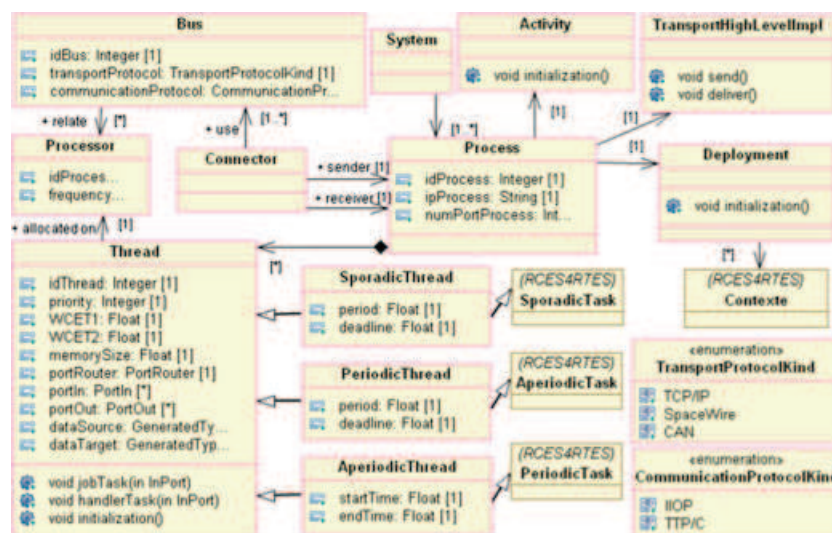
Figure 8. Implementation meta-model.
