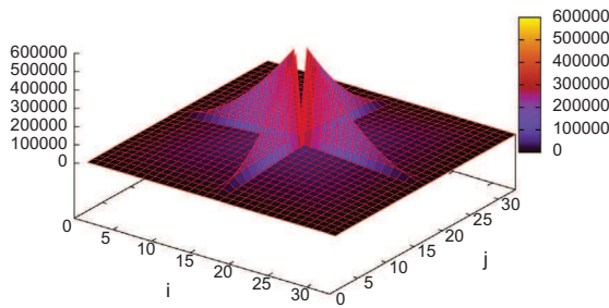
(a) Equiproportional routing
