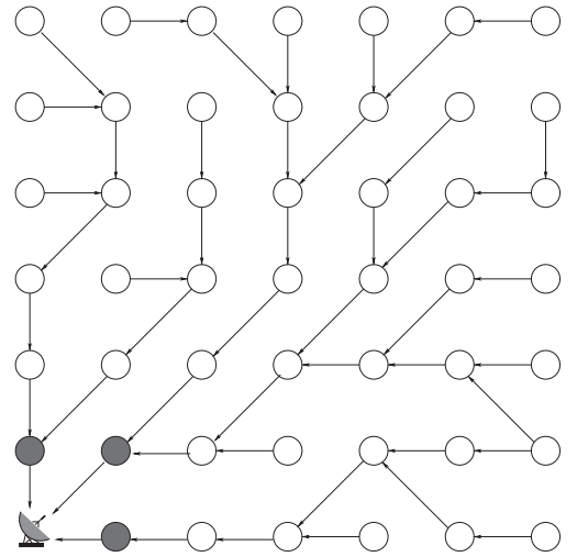
Fig. 1. A many-to-one traffic pattern impact in a 2-D grid topology with BS in the corner.
