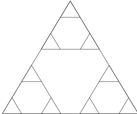
FIGURE 5. The case n = 3 . The largest disk is moved along the middle edge as in the case for n = 2 , but as n grows, the middle edge will take on a smaller and smaller proportion of the side of the triangle. Hence the graph representation of Tower of Hanoi will converge to the Sierpinski gasket, the minimal normal-play (EC1) path being along the base of the triangle.
