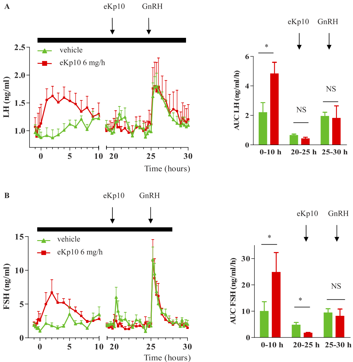
FIG. 6. Experiment 6: effects of acute eKp10 and GnRH injections during midterm perfusion of eKp10 in cyclic mares. A, B Left panels are plasma concentrations (mean \pm SEM) of LH and FSH during the 30 h of eKp10 at 6 mg/h (red symbols) or saline (green symbols) perfusion at early follicular phase. Mares received a single i.v. injection of eKp10 after 20 h (1 mg, first black arrow) followed by a single i.v. injection of GnRH (25 \mu g) 5 h later (second black arrow). The period of perfusion (30 h) is represented by a black bar. Right panels are AUC for LH and FSH during the 0–10 h period of perfusion of eKp10 at 6 mg/h or vehicle, and after eKp10 and GnRH bolus injections at, respectively, 20 and 25 h (same color code as for A ). * P < 0.05 , permutation test for independent samples with two-tailed P value. NS, not significant.
