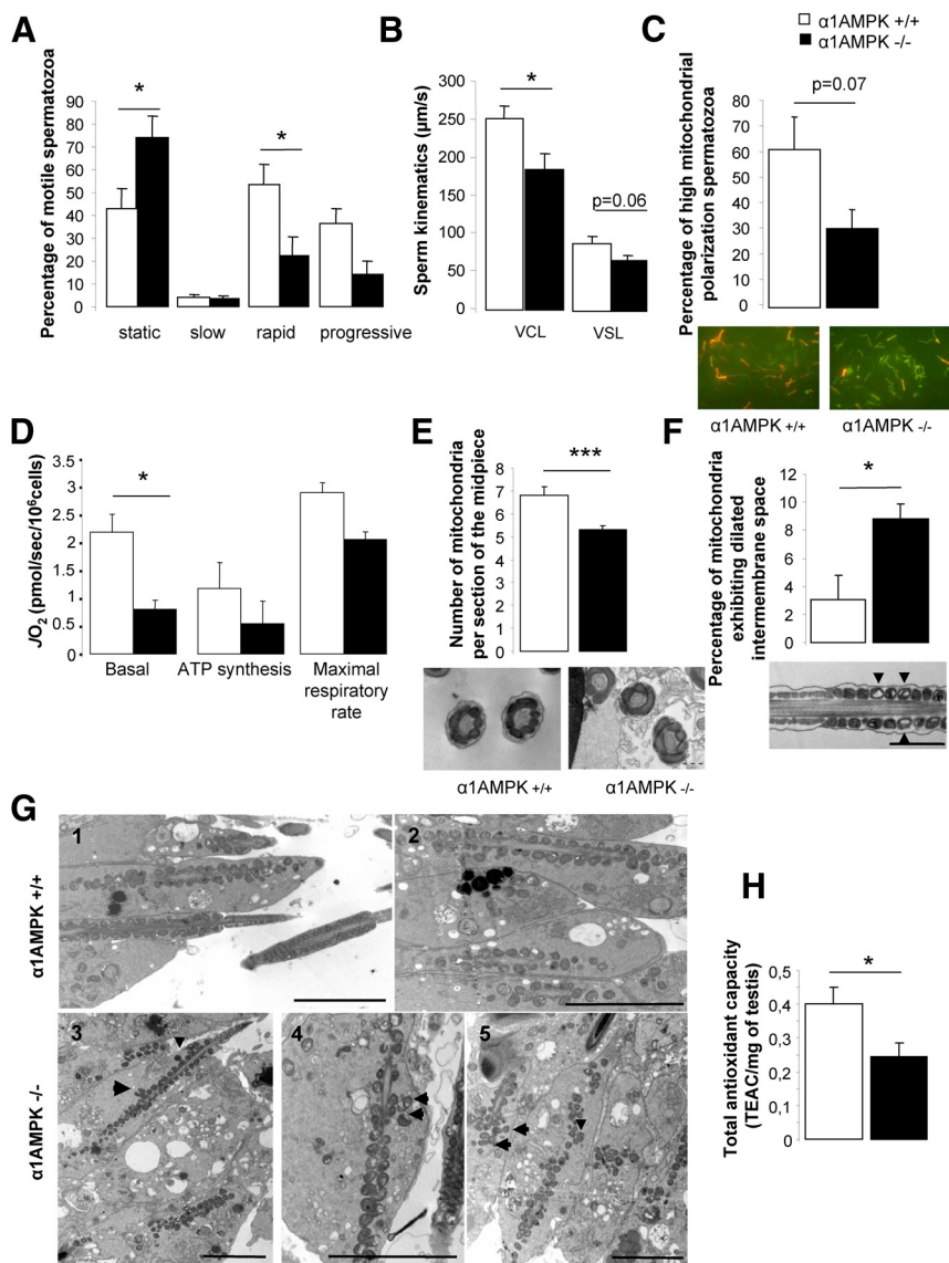
FIG. 4. Analysis of spermatozoa mobility and characterization of mitochondria. Sperm mobility parameters, percentage of motile spermatozoa (A) and sperm kinematics (B) of \alpha 1AMPK^{+/+} mice (n = 6) and \alpha 1AMPK^{-/-} mice (n = 6), were performed by computer-assisted sperm analysis. VCL, Sperm curvilinear velocity; VSL, sperm straight-line velocity. *, P < 0.05 . C, Mitochondrial activity was determined by JC-1 staining and represented by percentage of high mitochondrial polarization spermatozoa (orange/red fluorescence) in \alpha 1AMPK^{+/+} mice (n = 5) and \alpha 1AMPK^{-/-} mice (n = 5). Low mitochondrial membrane potential was observed in green fluorescence. D, Spermatozoa suspension ( 2 \times 10^6 cells/ml) in M2 medium supplemented with 5 mM sodium pyruvate was transferred immediately, after isolation, into a stirrer 2-ml oxygraph vessel where JO_2 was recorded before and after the successive addition of 0.5 \mu g/ml oligomycin and 1–2 \mu M carbonyl cyanide m -chlorophenylhydrazone. Data are represented as means \pm SEM of n = 3 different spermatozoa isolations in which measurements were performed in duplicate. *, P < 0.05 . E, The number of mitochondria per section of spermatozoa in the midpiece from \alpha 1AMPK^{+/+} mice (n = 5) and \alpha 1AMPK^{-/-} mice (n = 5). Scale bar, 500 nm. F, Percentage of mitochondria exhibiting partial or total cristolysis was measured on transmission electron micrographs. Black arrows indicate cristolysis in mitochondria. Scale bar, 1 \mu m . G, Testis micrographs from \alpha 1AMPK^{-/-} mice (3–5) exhibited abnormal arrangement of mitochondria (arrowhead) during midpiece formation in the testis compared with \alpha 1AMPK wild-type mice (1 and 2). Scale bar, 5 \mu m . H, Intratesticular antioxidant activity measured in units called Trolox equivalent antioxidant capacity (TEAC) per milligram of testis. Data are represented as mean or percentage \pm SEM. *, P < 0.05 ; ***, P < 0.001 .
