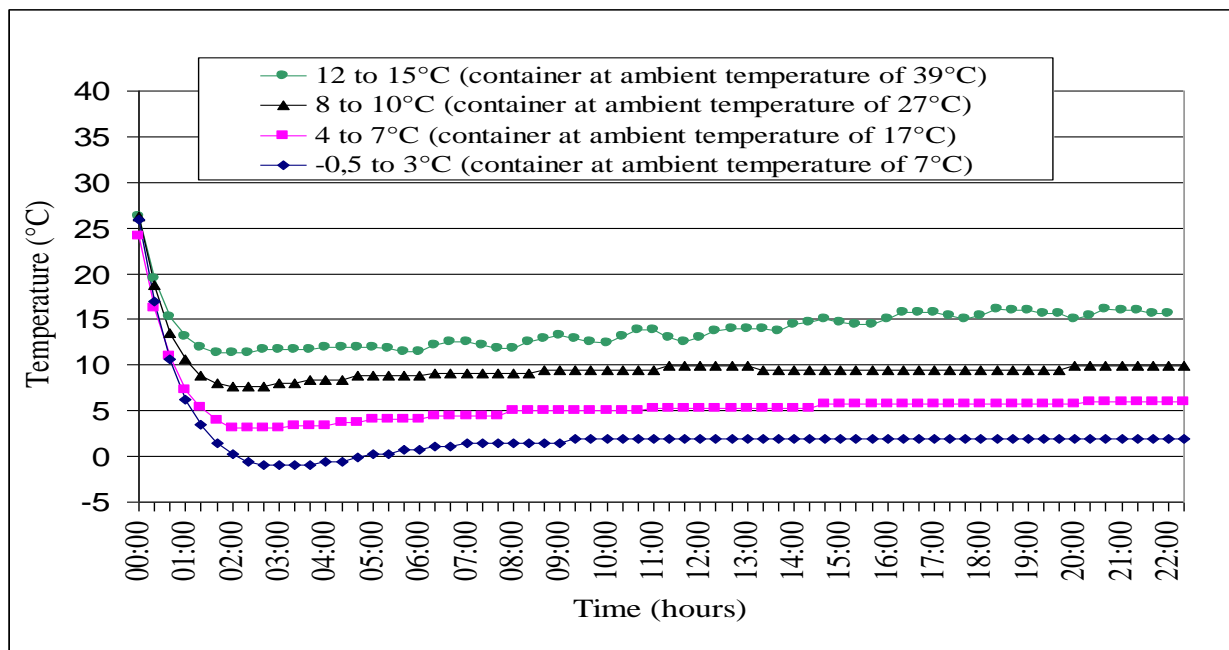
Figure I : Temperature curves in the sperm dose loaded in the disposable container placed at different ambient temperatures, after samples reached 25°C (Experiment 2). Each bar on x axis represents 20 min. Lowest temperature was obtained in 2 h 50 min, 2 h 30 min, 2 h 20 min and 2 h 00 min, in container stored at 7, 17, 27 and 39°C, respectively.
