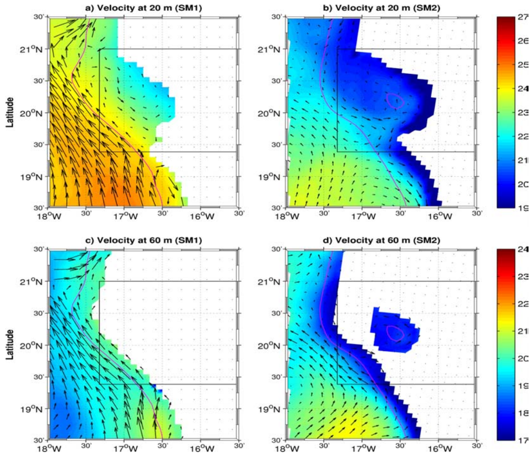
Figure 11 – Temperature ( ^{\circ}\text{C} ) and horizontal current ( \text{cm s}^{-1} ) at 20 m (top) and 60 m (bottom) depths for SM1 (left) and SM2 (right) in December for the northern area.
