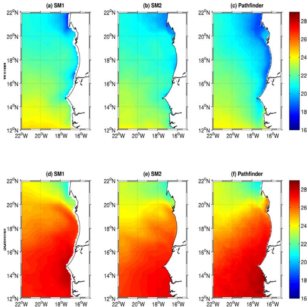
Figure 2 – Sea Surface Temperature (SST, °C) during winter (January-March) (top) and summer (July-September) (bottom) for SM1 (a,d), SM2 (b,e) model output, and Pathfinder observations (c,f).
