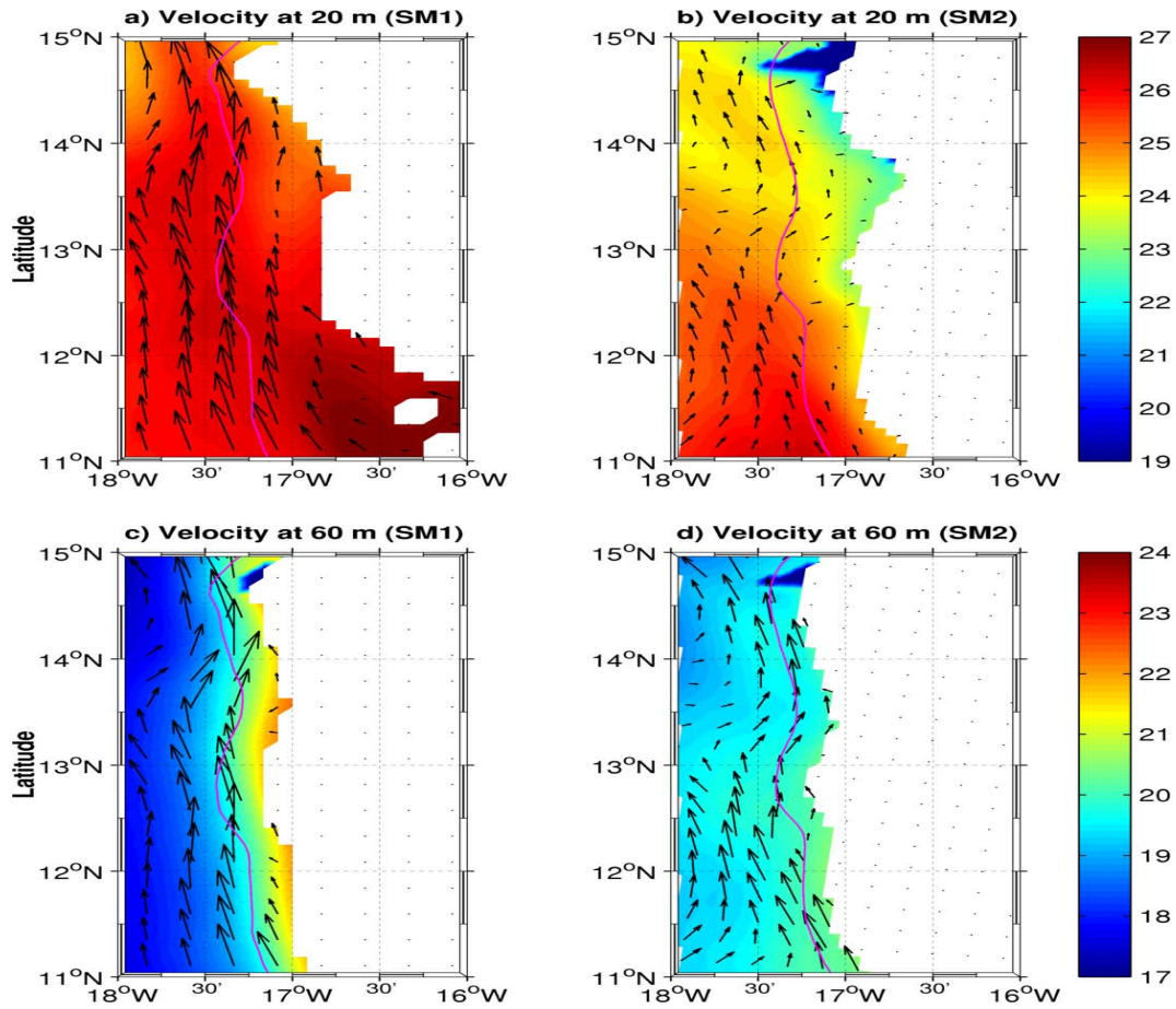
Figure 13 – Same as Figure 3.14, in June for the southern area.
