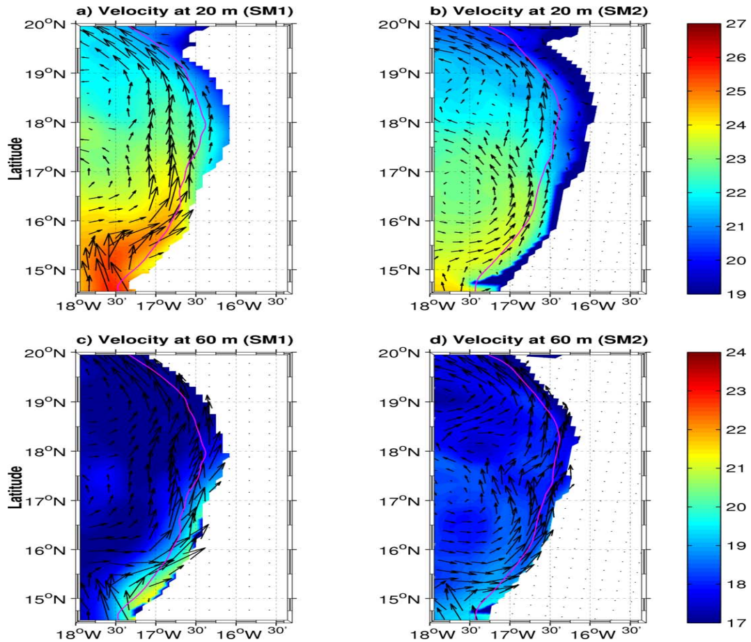
Figure 12 – Same as Figure 3.14, in June for the central area.
