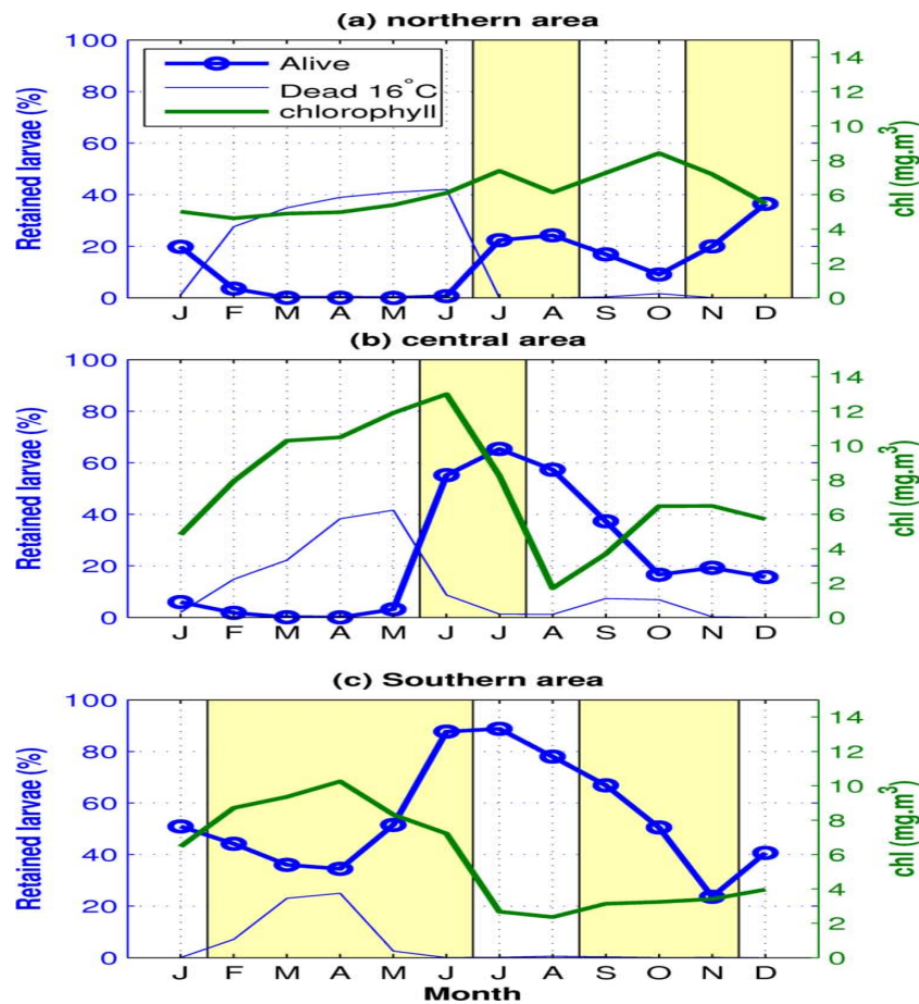
Figure 14 – SeaWIFS surface chlorophyll ( \text{mg Chl m}^{-3} , green line) averaged between the coast and the 200 m isobath, retention of living (thick blue line with round marks) and dead (thin blue line) larvae for the northern (a), central (b) and southern (c) areas. Experiment using DVM60 and a lethal temperature of 16^{\circ}\text{C} are shown. Yellow rectangles indicate a priori observed spawning periods.
