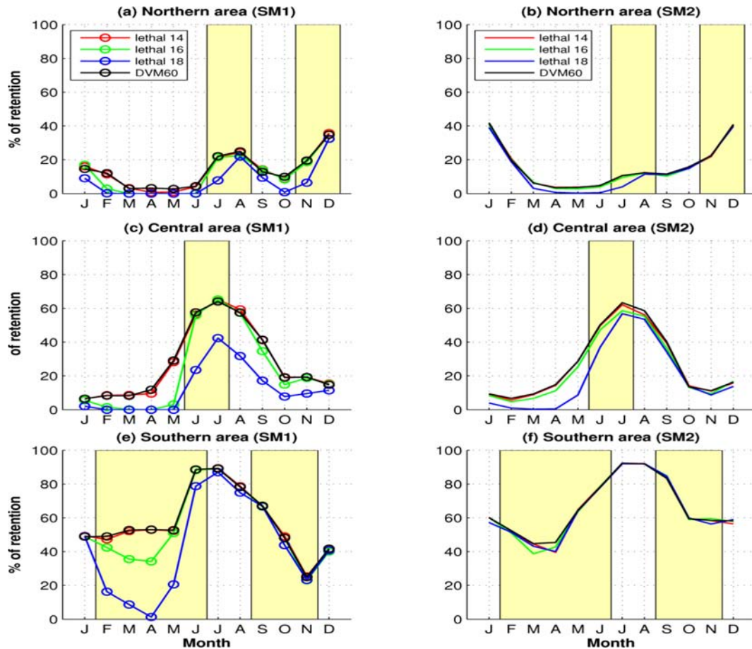
Figure 6 – Seasonality of shelf retention rates (% of larvae) in the case of different lethal temperature thresholds : 14°C (red line), 16°C (green line) and 18°C (blue line). Experiments were achieved following a DVM60 scenario for the northern (a,b), central (c,d) and southern (e,f) areas. DVM60 without any temperature effect is shown in black. SM1 and SM2 model results are shown in the left and right columns respectively. Yellow rectangles indicate a priori observed spawning periods.
