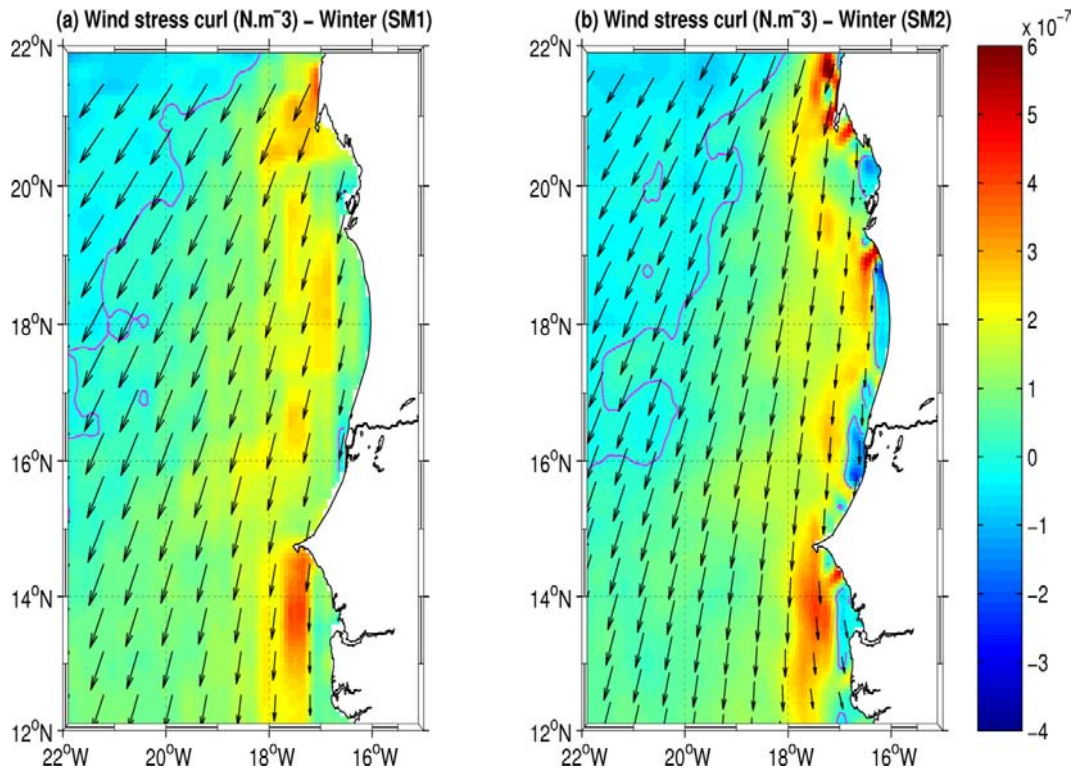
Figure 8 – Wind stress (arrows, N.m^{-2} ) and wind stress curl (colors, N.m^{-3} ) from the different products (see text) forcing SM1 (a) and SM2 (b) simulations during winter (January-March). The zero wind stress curl is contoured in blue.
