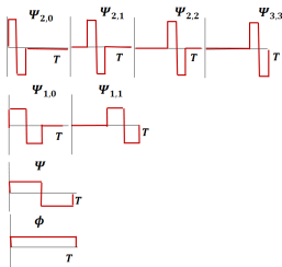
Figure 7: Haar wavelet function for different scales.
