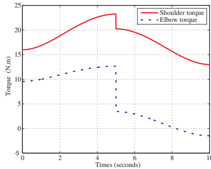
Figure 6: Shoulder and elbow joint torques \Gamma_{\text{joint}} for one operating cycle. The first phase is a pushing phase
